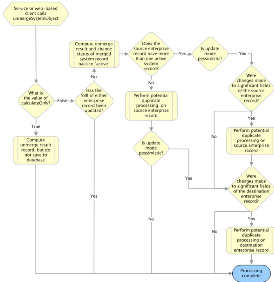
Figure 2–17 unmergeSystemObject Processing
