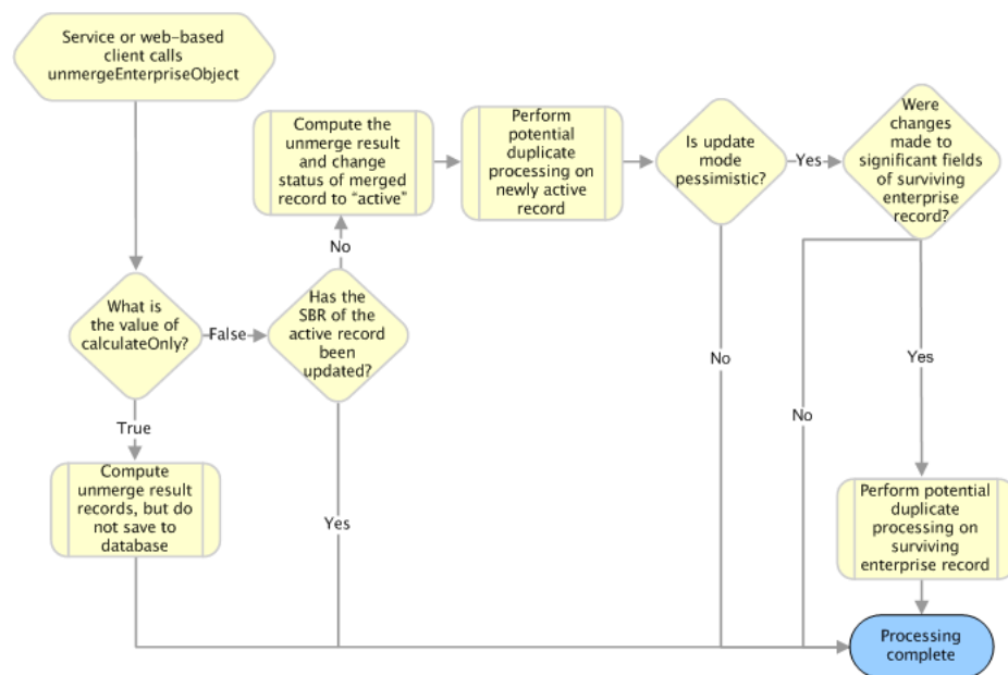
Figure 2–16 unmergeEnterpriseObject Processing
