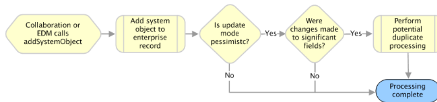
Figure 2–9 addSystemObject Processing
