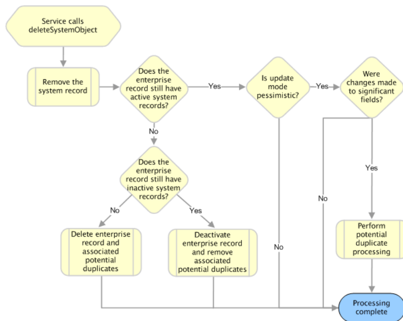
Figure 2–11 deleteSystemObject Processing
