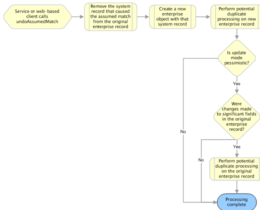
Figure 2–15 undoAssumedMatch Processing
