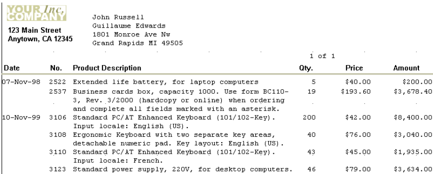
Figure 3-30 Final output of the preprinted forms example
