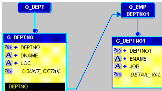
Figure 21–3 Data Model view with formula and summary columns
