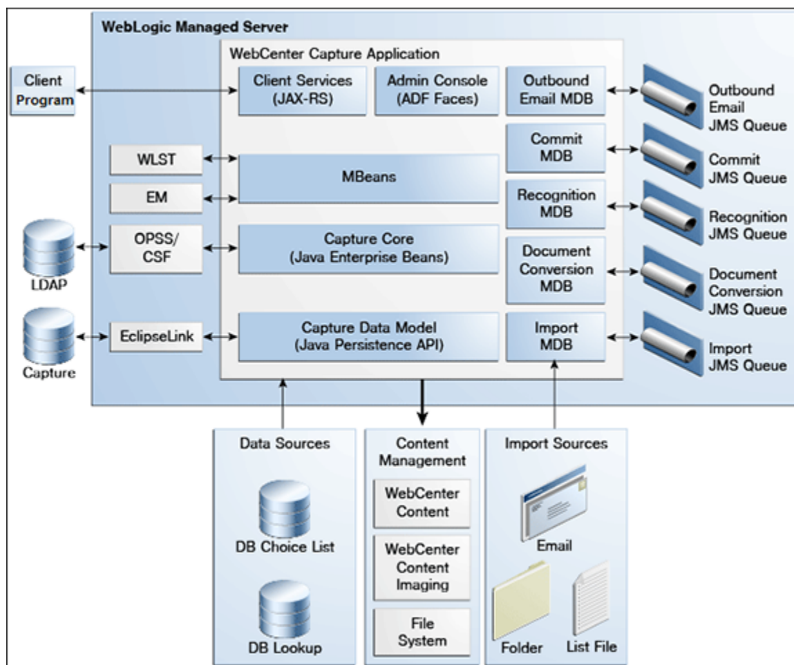
Figure 2-1 Oracle WebCenter Enterprise Capture Architecture Overview
