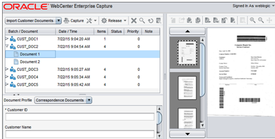
Figure 2-2 Capture Client Window Displaying Batch, Document, and Metadata Panes
