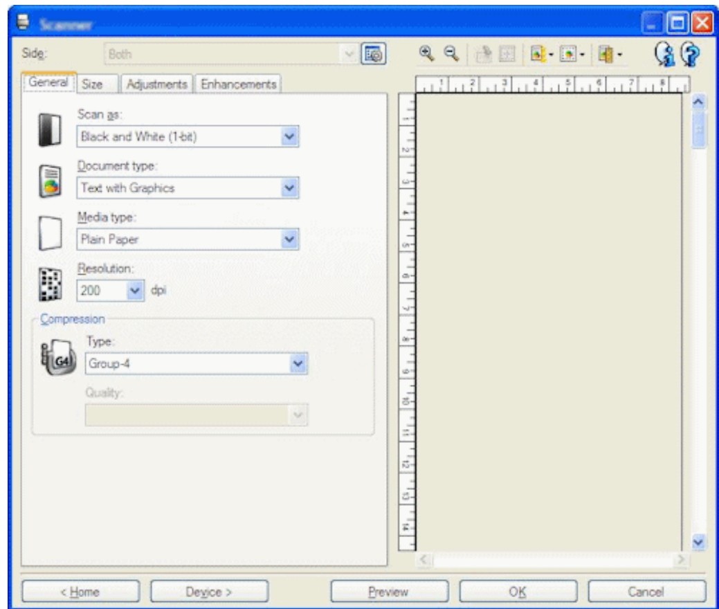
Figure 3-1 Example Scanner Settings
