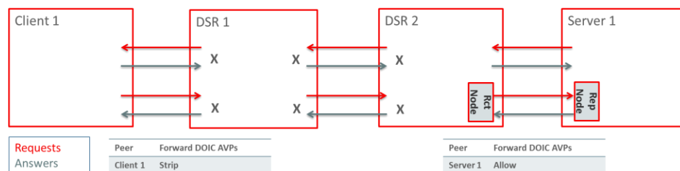
Figure 31 - DOIC Security Setting Example
