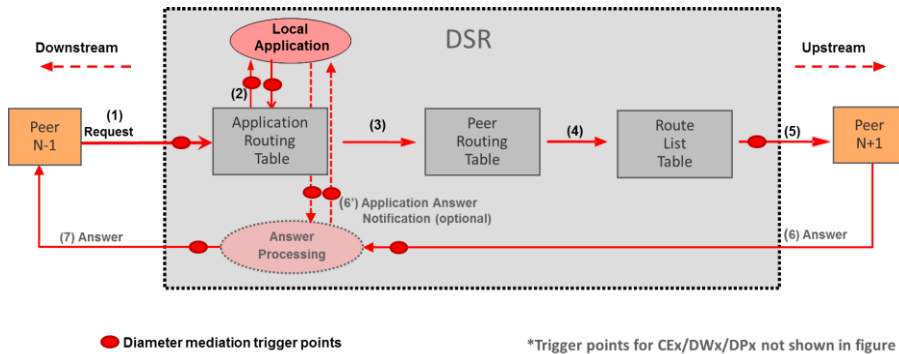
Figure 46 - Mediation Trigger Points
