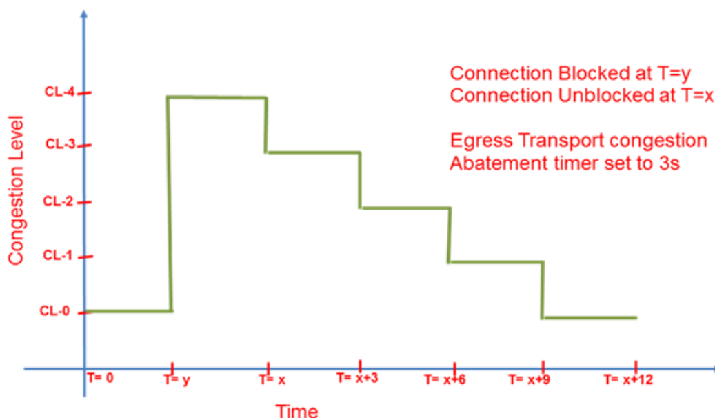
Figure 22 – Example Congestion level abatement
