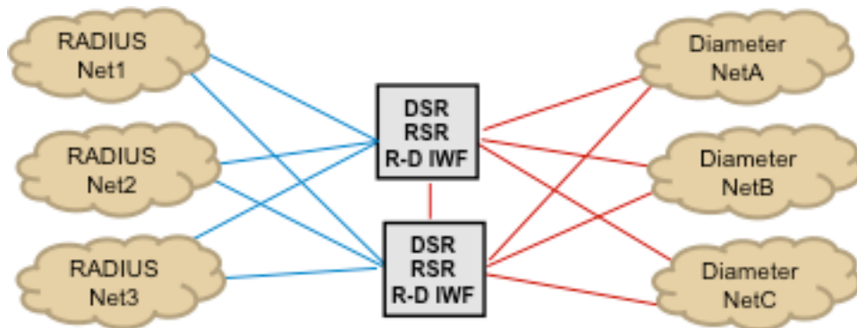
Figure 44 - RSR and R-D IWF Deployment
