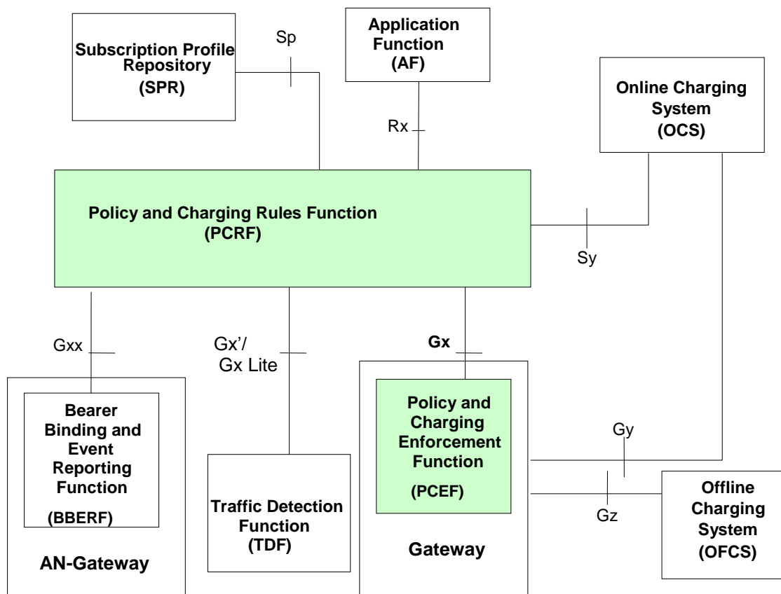
Figure 56 - Overall PCC logical architecture (non-roaming)
