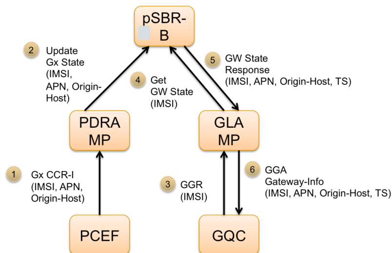
Figure 61 - IMSI Query with Single Matching Gx Session Use Case
