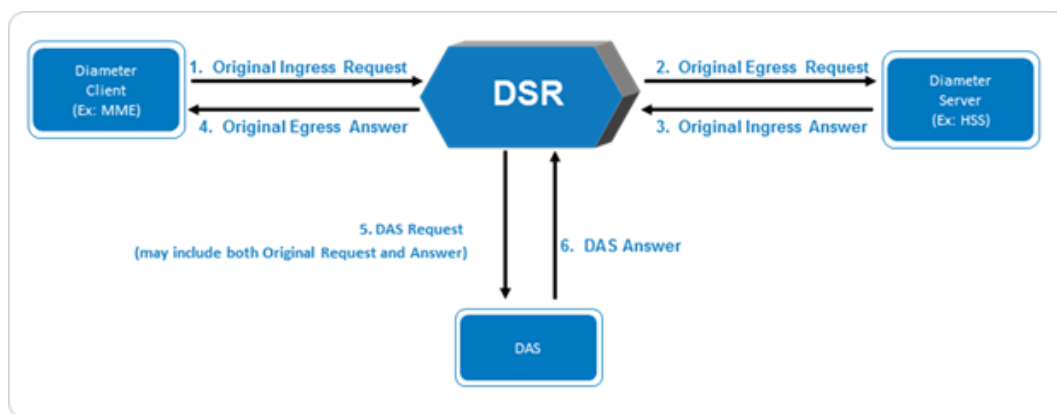
Figure 63 - Message Copy Overview
