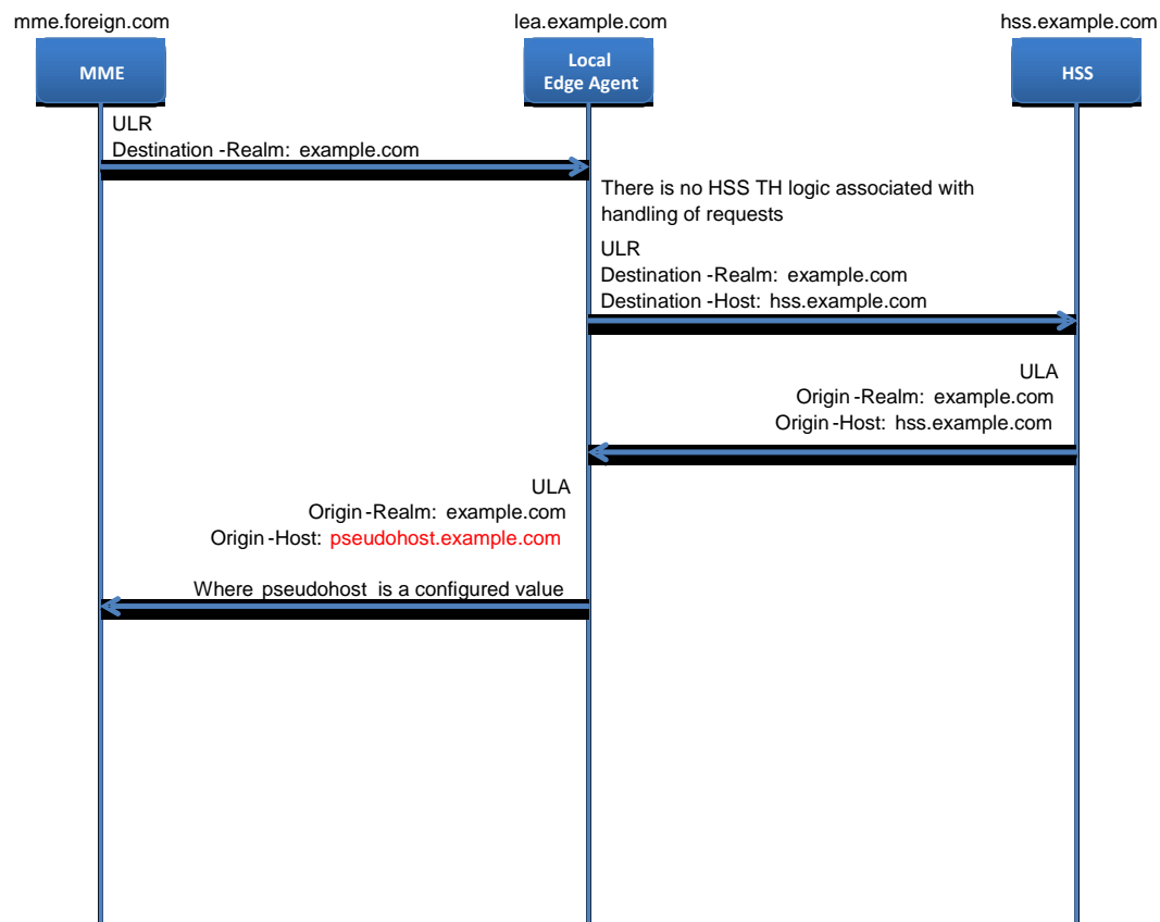
Figure 48 - S6a/S6d HSS Topology Hiding - ULR Message Flow
