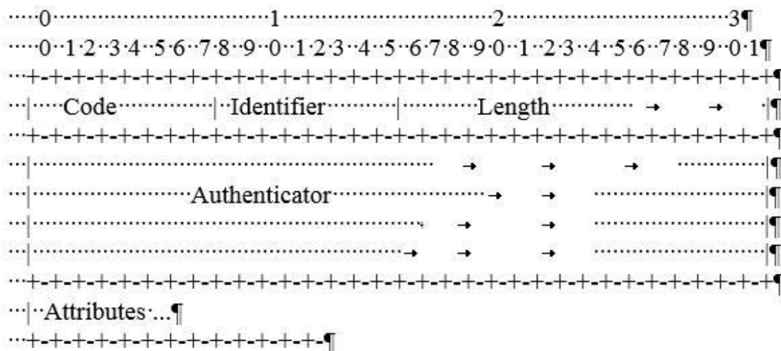
Figure 42 – RADIUS Data Format
