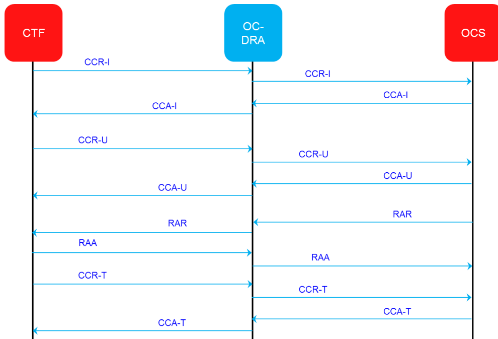
Figure 54 - A typical Online Charging Session
