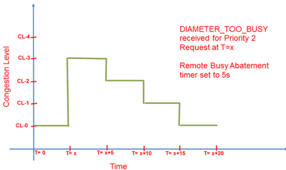
Figure 27 – Congestion level abatement over time for Remote Busy
