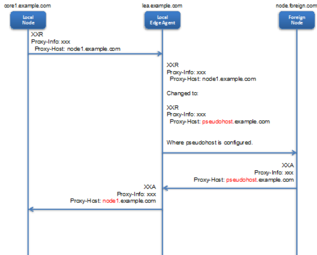
Figure 50 - Proxy-Host Topology Hiding Message Flow
