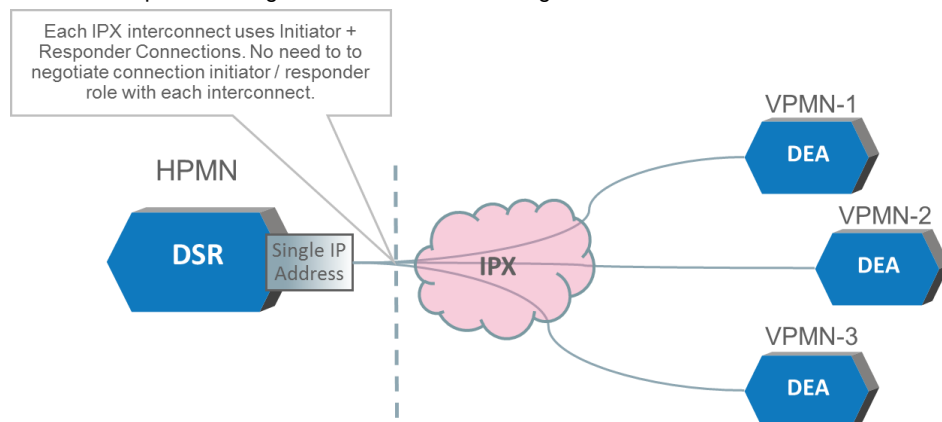
Figure 40 - IPFE Initiator + Responder Support
