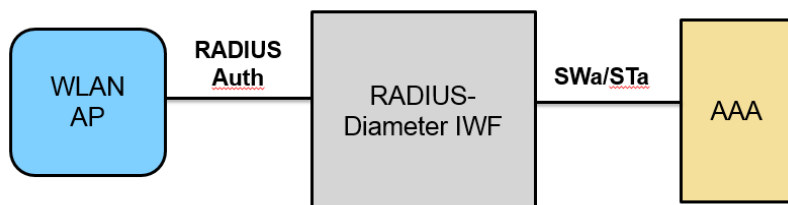
Figure 43 - RADIUS-Diameter IWF for WLAN Authentication
