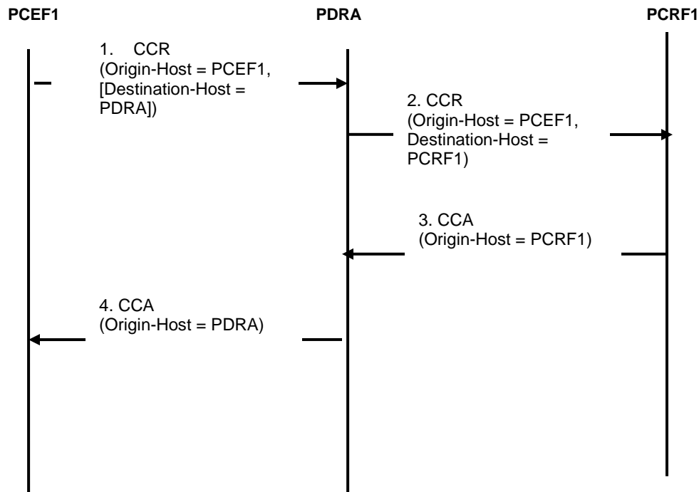
Figure 57 - PCRF topology hiding
