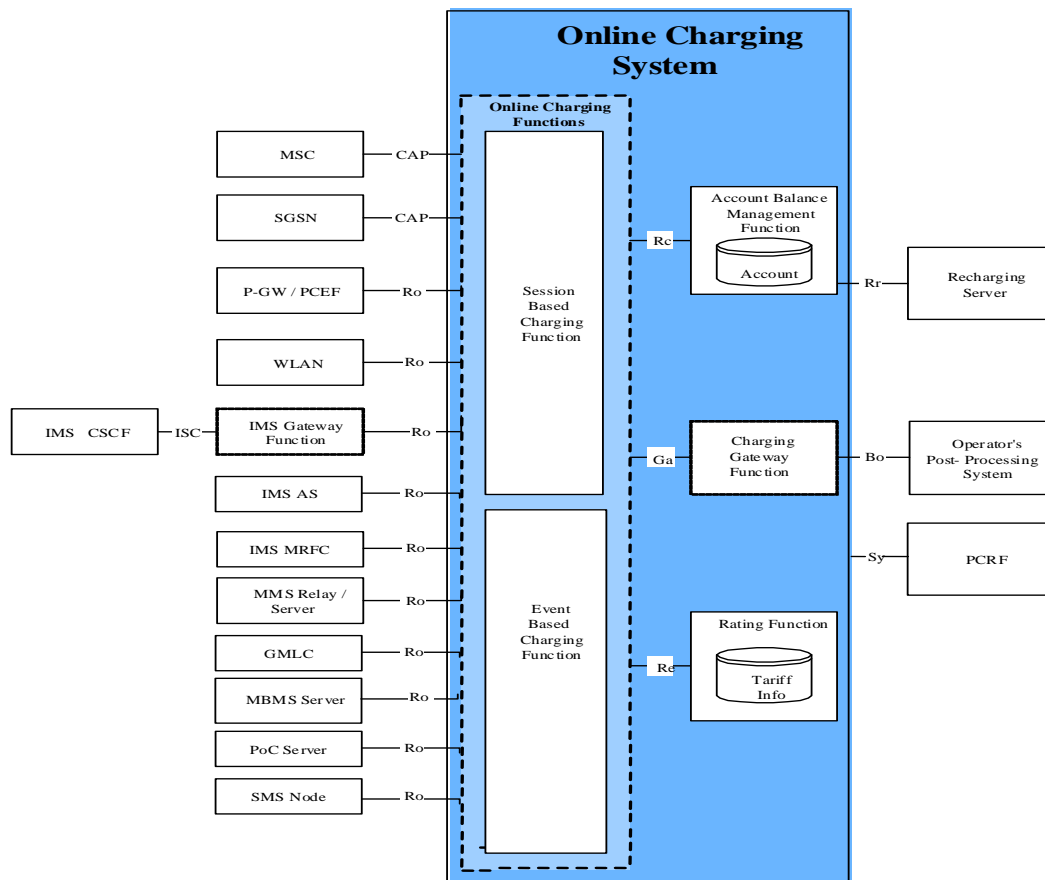
Figure 53 - Online Charging System and Architecture
