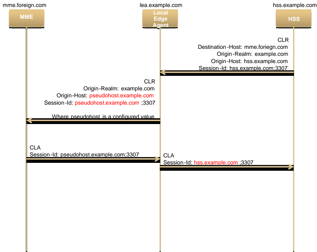
Figure 49 - S6a/S6d HSS Topology Hiding CLR Message Flow
