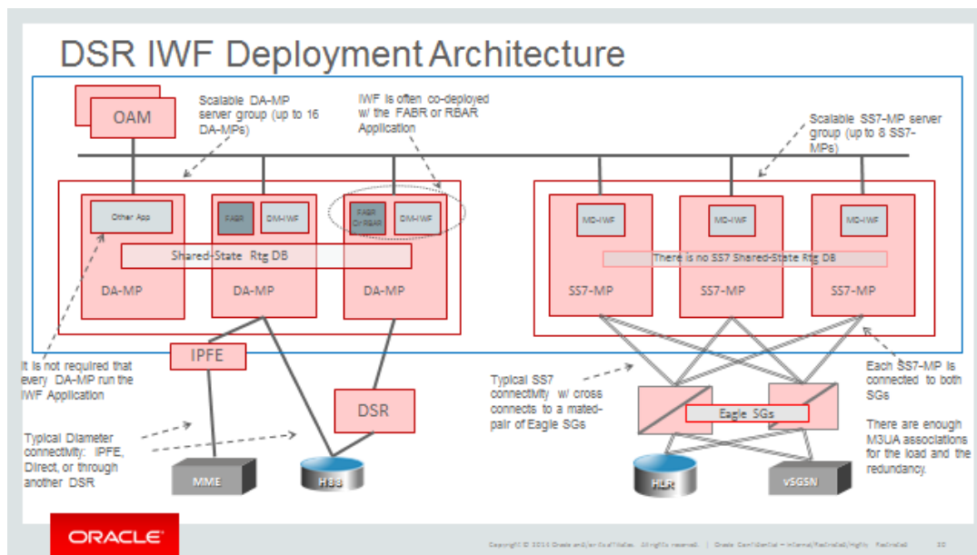
Figure 52 - DSR with MAP-Diameter IWF
