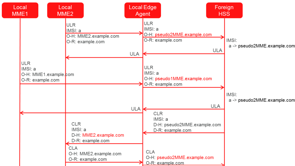
Figure 47 - MME/SGSN Topology Hiding
