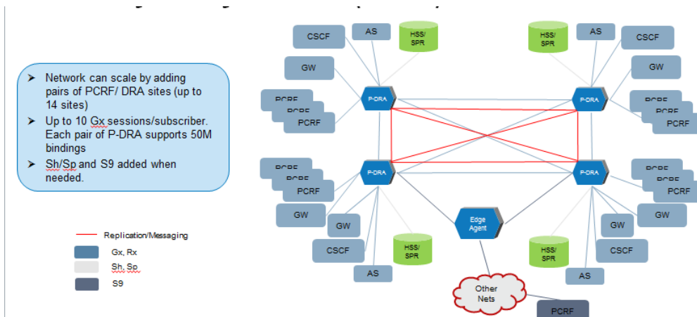
Figure 60 - PCA Example Deployment
