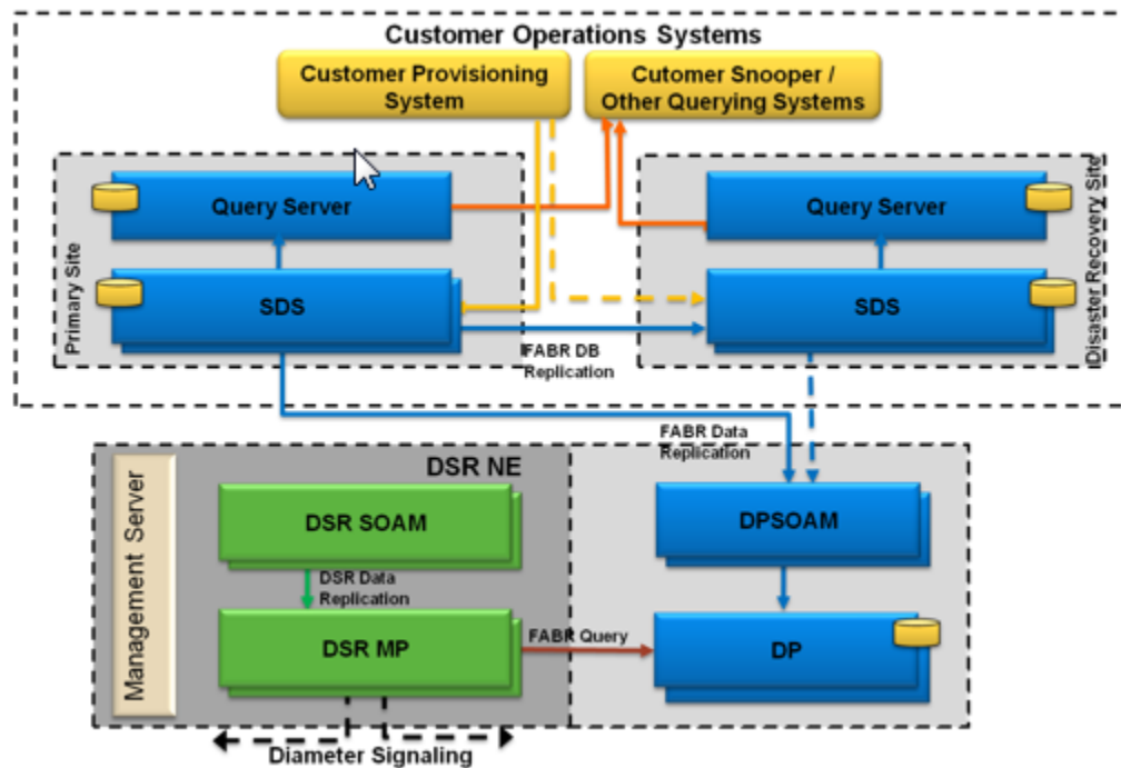
Figure 51 - Subscriber Data Server Architecture
