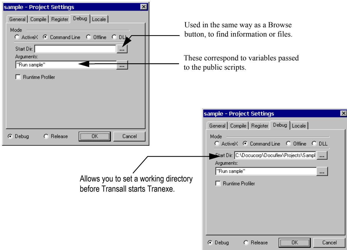
Figure 191: Command-line Debug Settings in the Project Settings Dialog
