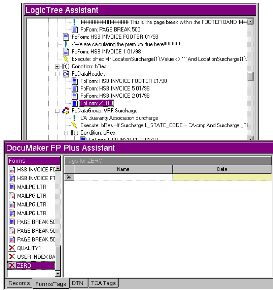
Figure 128: New Form without Tags
