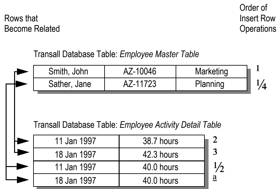
Figure 174: Connected Rows for Parent Table and Child Table
