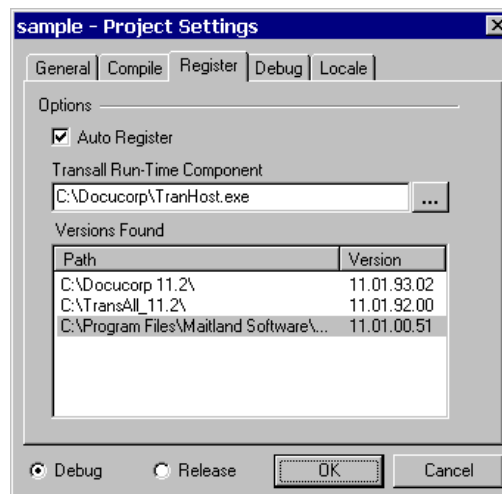
Figure 187: Register Settings in the Project Settings Dialog
