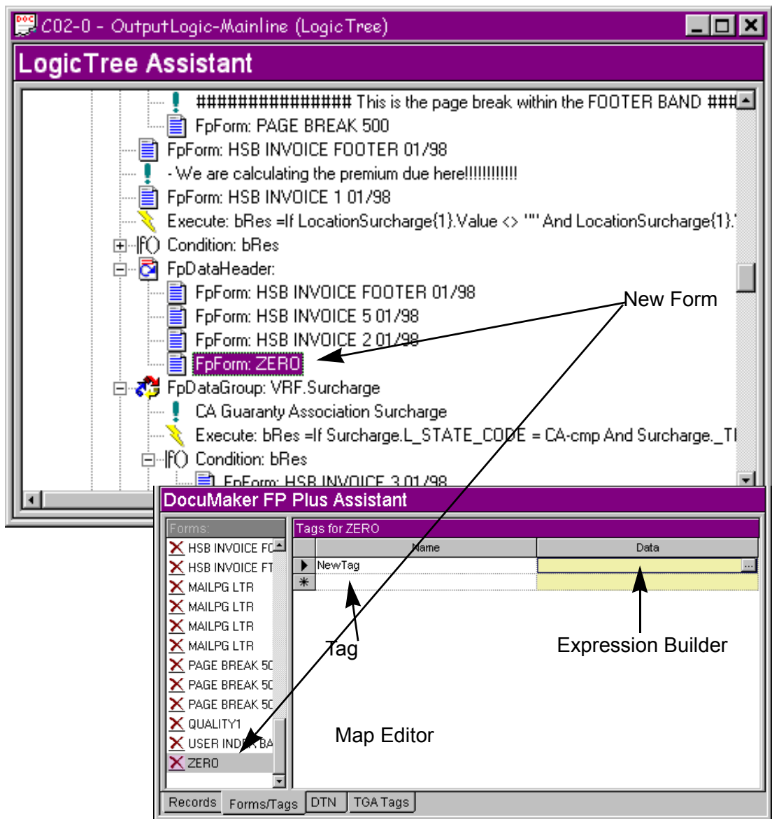
Figure 125: New Form with Tags
