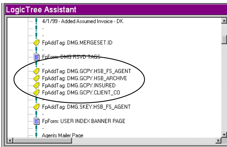
Figure 132: Example of FpAddTag
