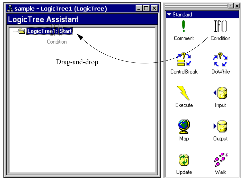
Figure 177: Dragging New Instruction into the LogicTree Assistant
