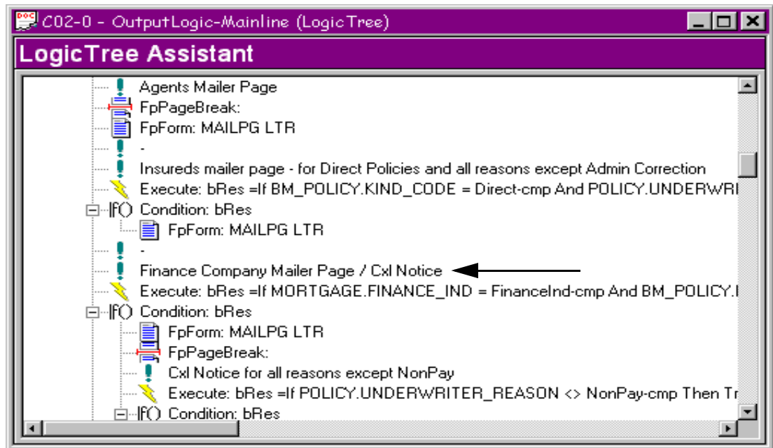
Figure 112: Example of a FpComment
