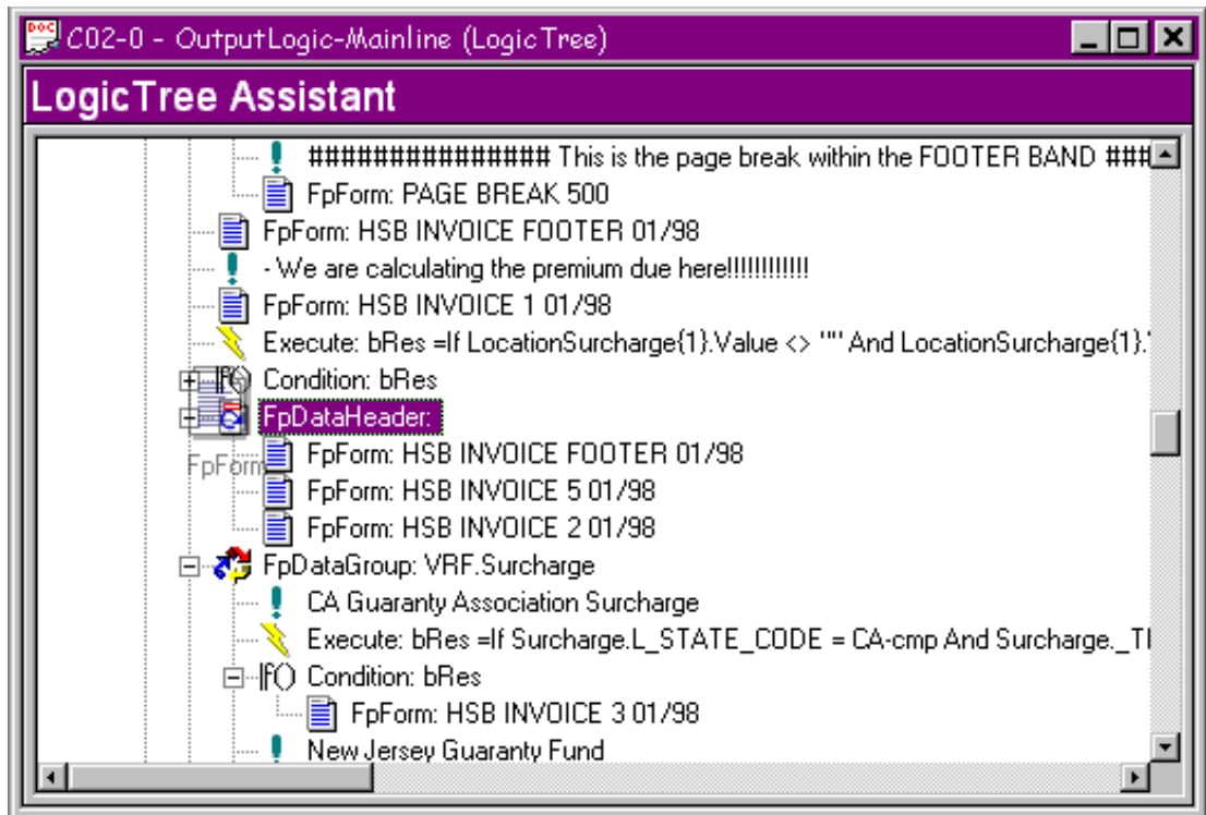
Figure 115: FpForm in LogicTree Assistant
