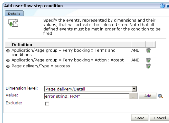
Figure 9–3 Add User Flow Step Condition
