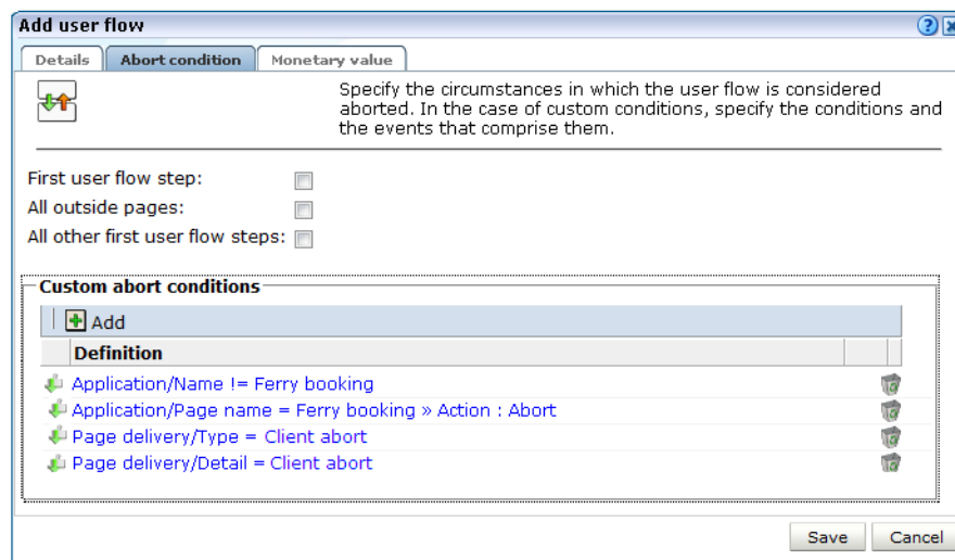
Figure 9–4 User Flow Abort Conditions Section
