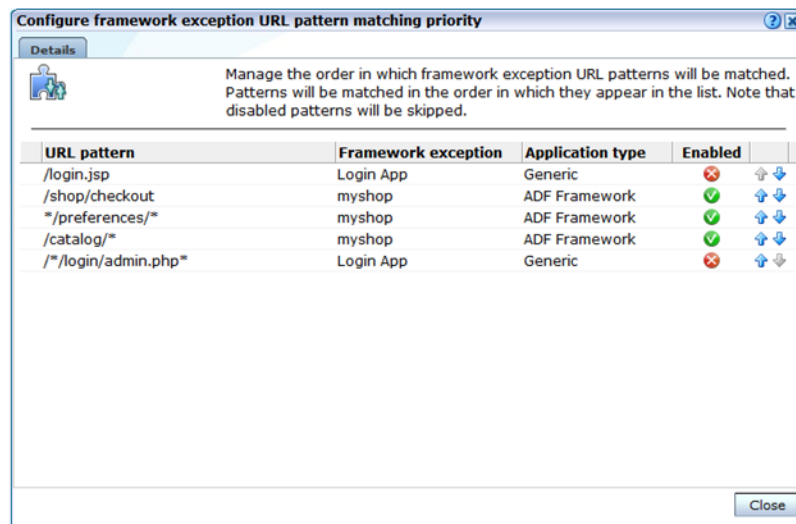
Figure 10–14 Framework Exception Priority Window
