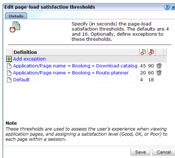
Figure 7–20 Edit Page-Load Satisfaction Thresholds Dialog
