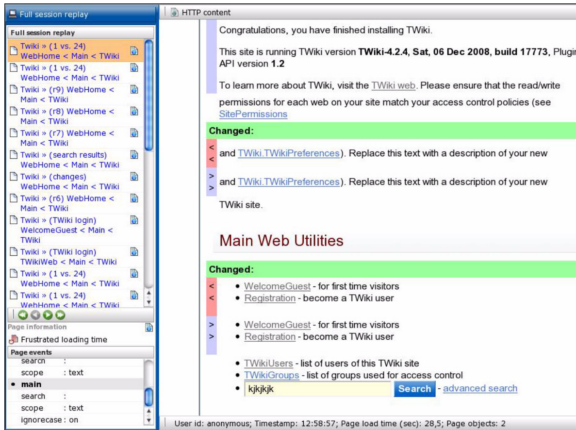
Figure 4-8 Example Session Replay
