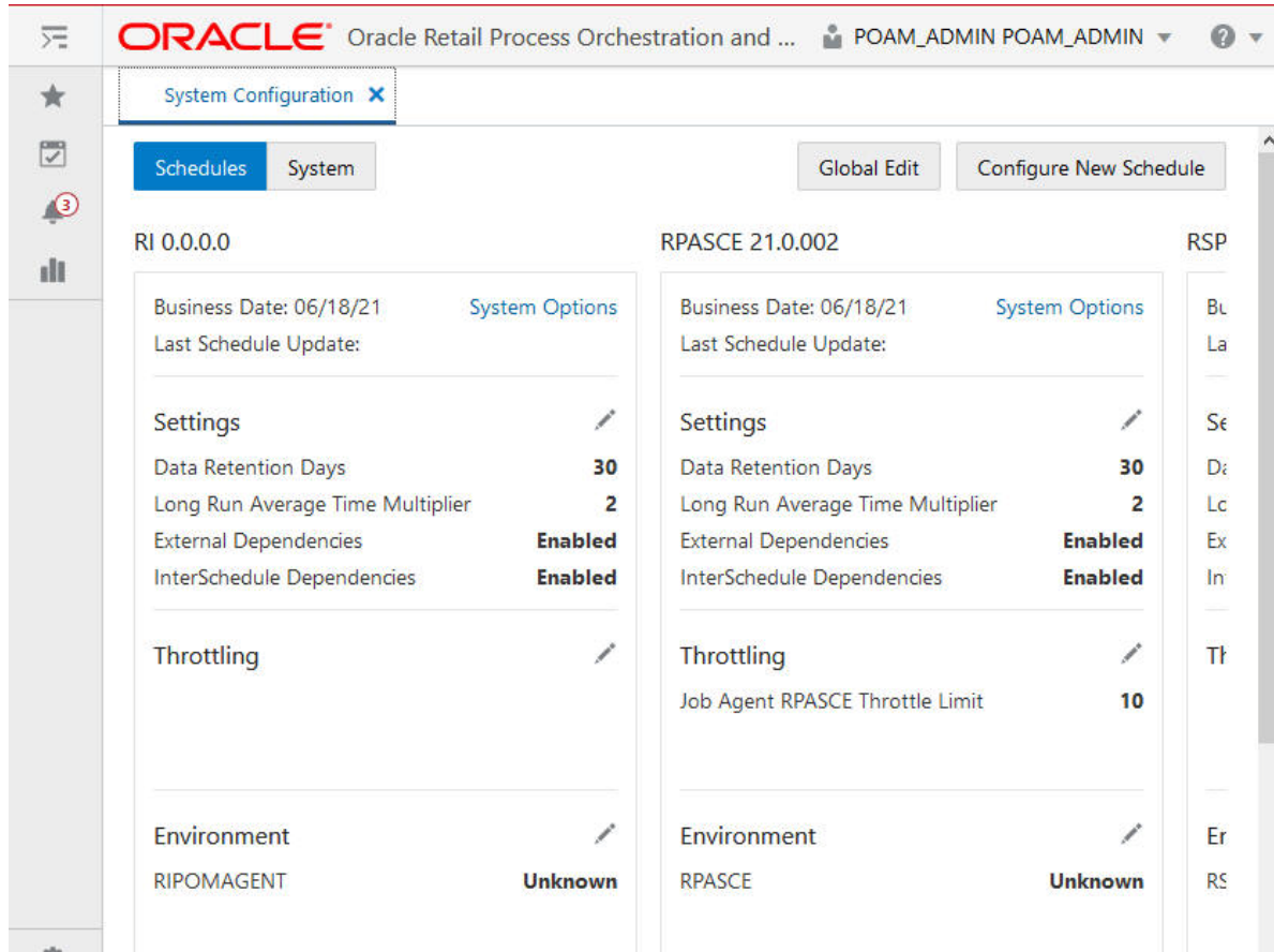
Figure 8–2 POM System Configuration
