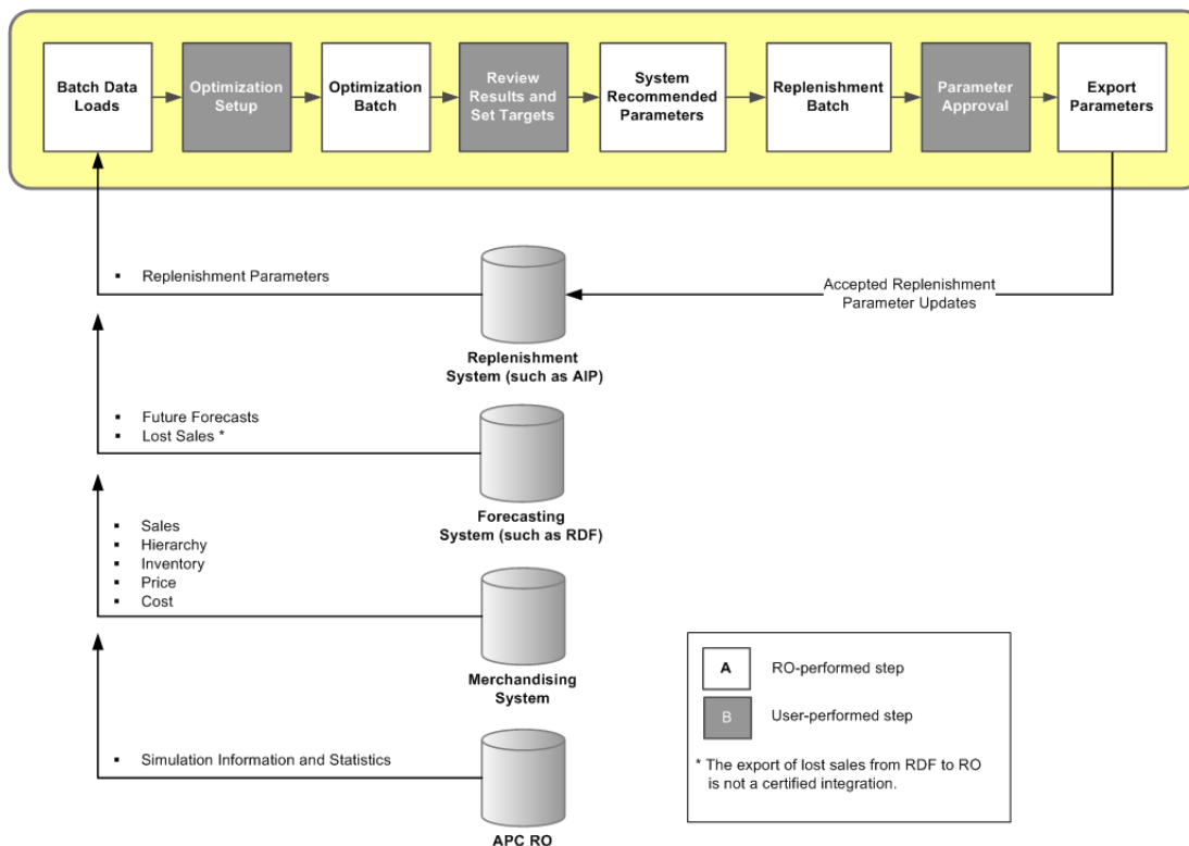
Figure 1–1 RO Solution Process Flow
