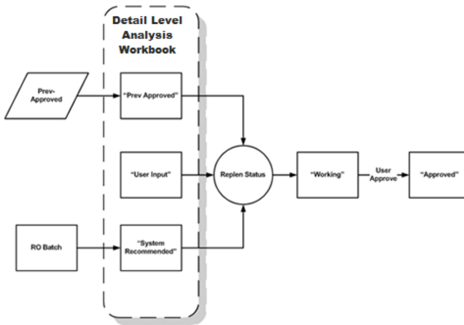
Figure 6–20 Approval Process Workflow in Detail Level Analysis
