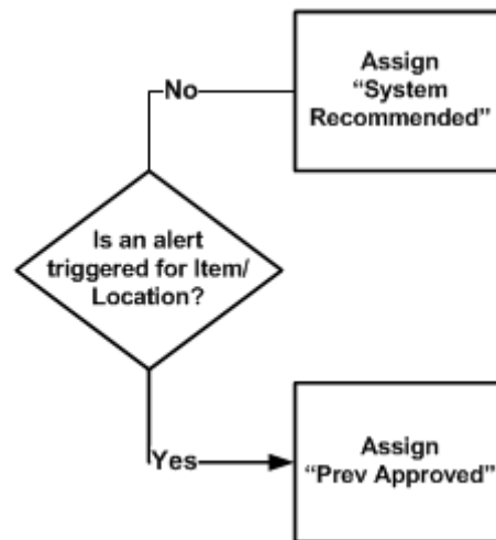
Figure 6–19 Default Replenishment Status Assignment
