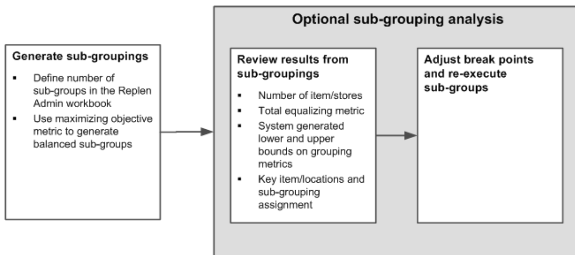
Figure 4-1 Subgroup Analysis Workbook User Process Flow
