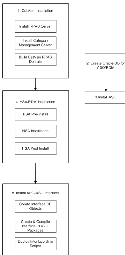
Figure 5–1 Assortment Planning and Optimization-ASO Integration Steps and Dependencies
