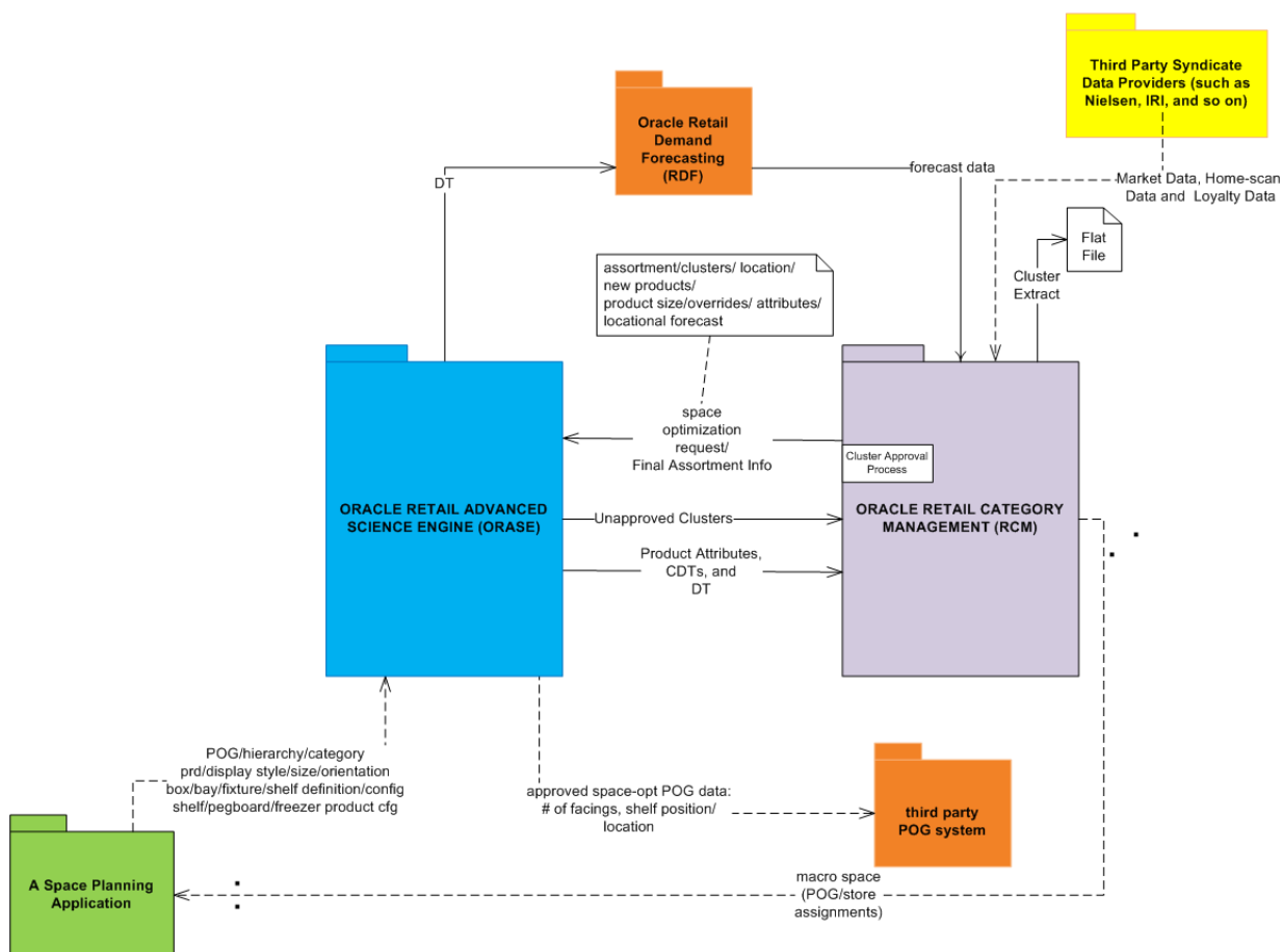
Figure 4–1 Category Management Data Flow
