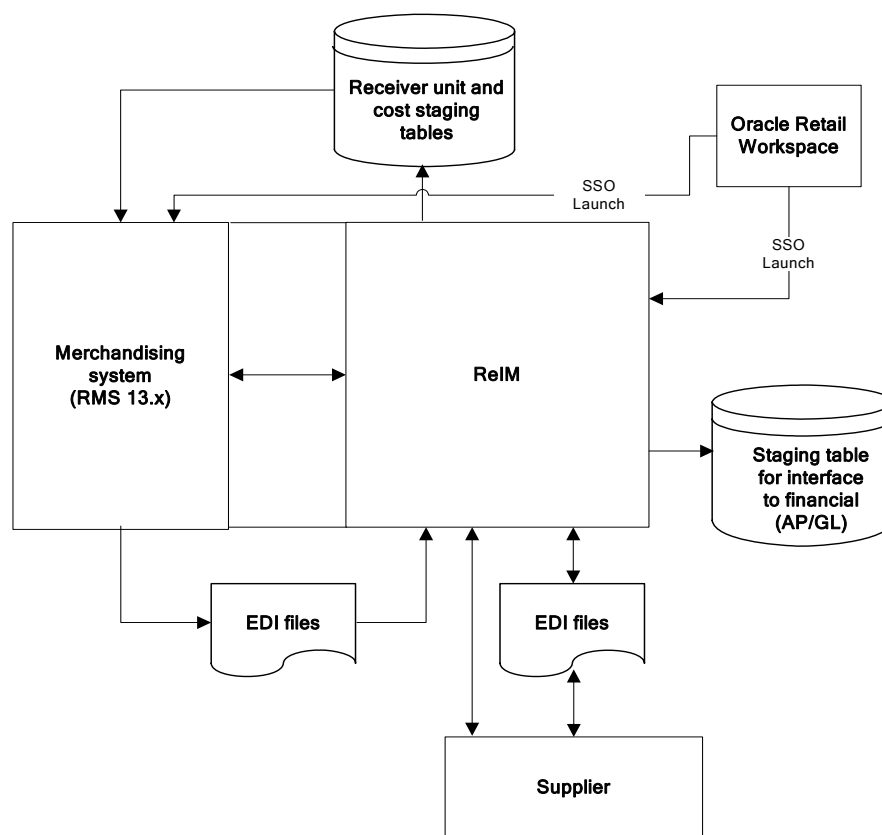
ReIM Dataflow across the Enterprise
