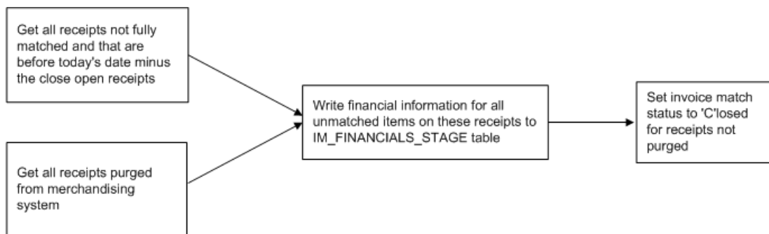
Figure 8–2 ReIM Receipt Write-Off Flow
