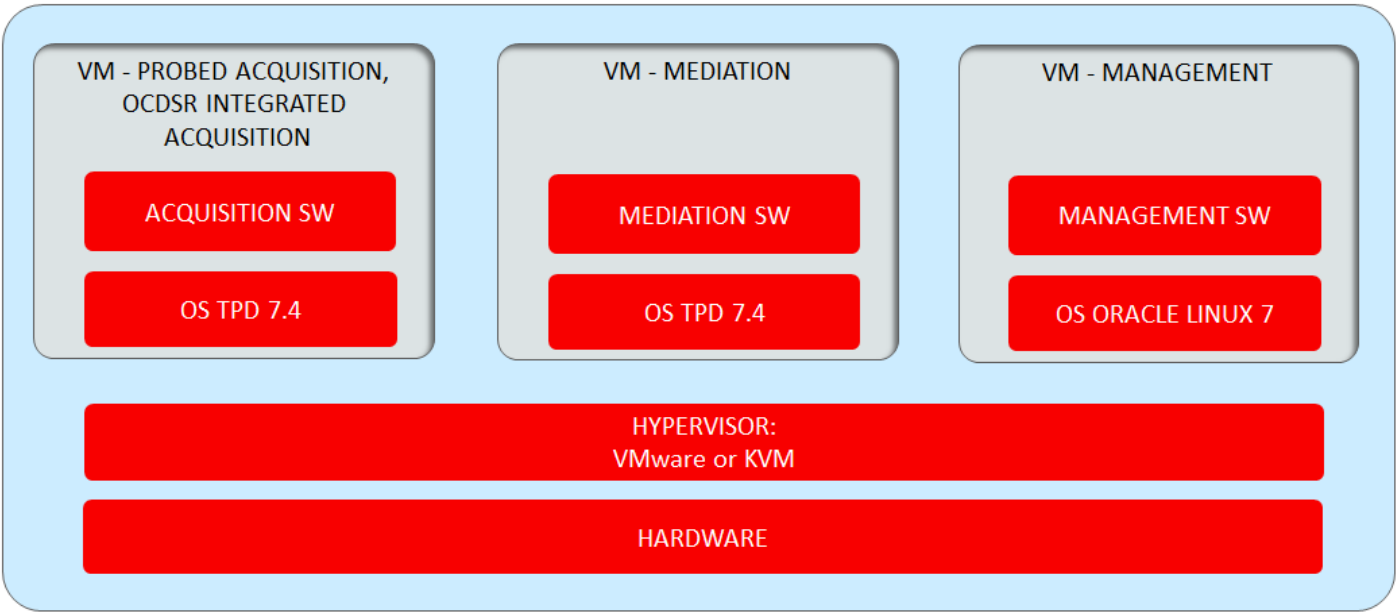
Figure 19 – Performance Intelligence Center Virtualization configurations
