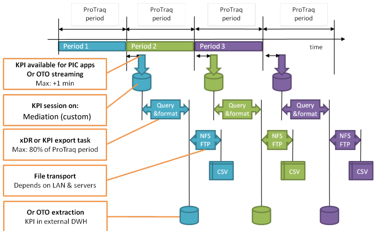
Figure 16 – Data Record & KPI Latency for applications and feeds
