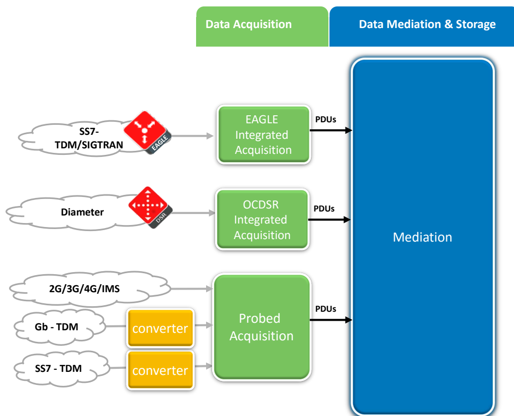
Figure 4 – Acquisition Configurations
