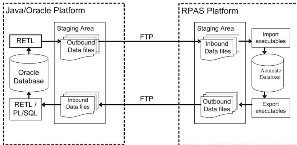
Figure 2-3 AIP Interfaces
