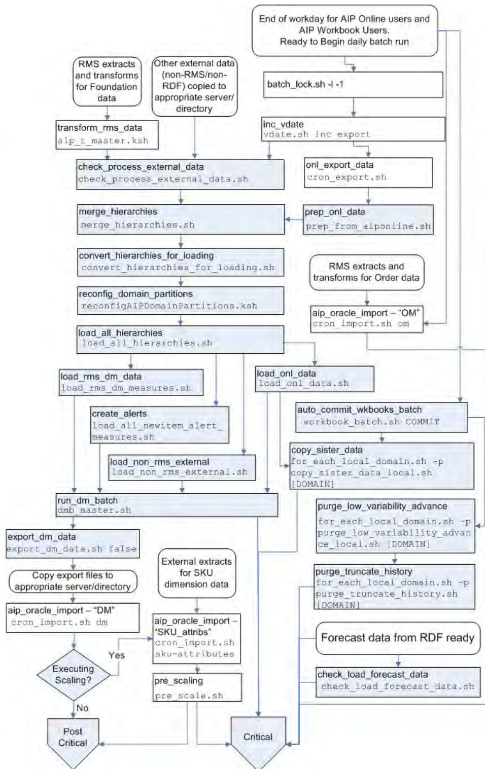
Figure 4-1 Pre-Critical Tasks Process Flow Diagram
