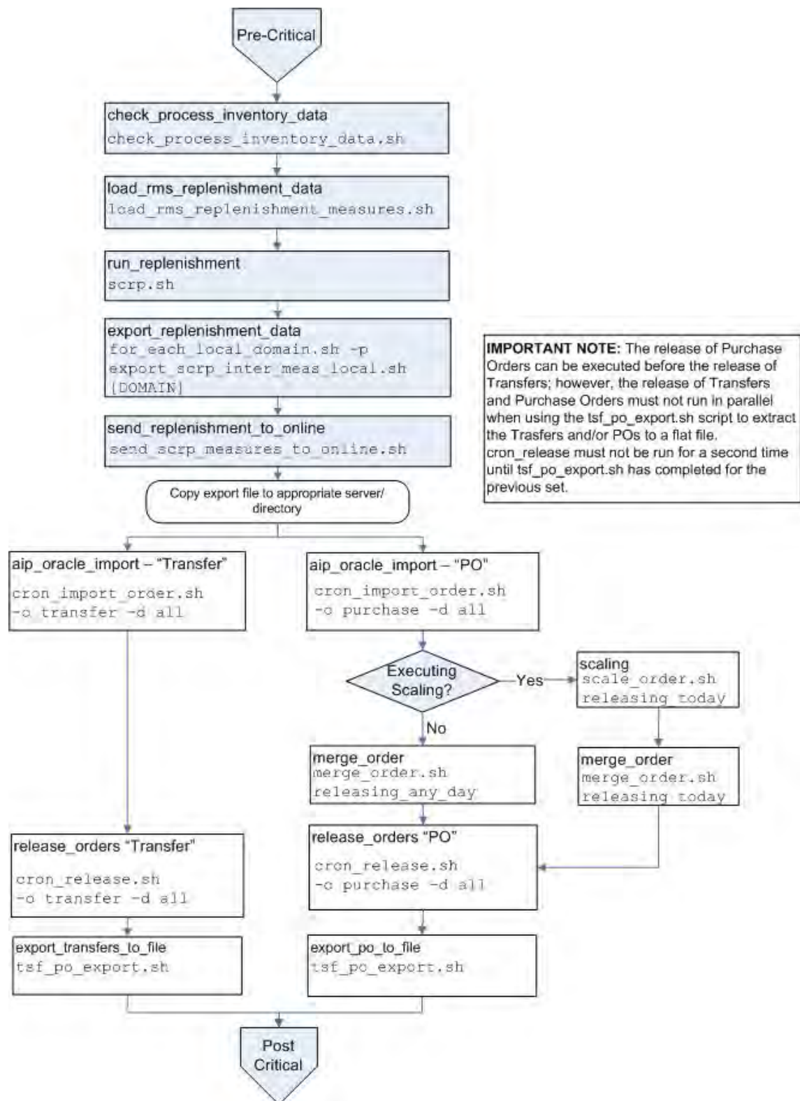
Figure 4-2 Critical Path Tasks Process Flow Diagram
