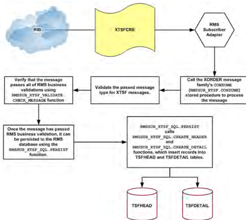
Figure 15–8 AIP Transfer Messages - RMS Load Process Diagram
