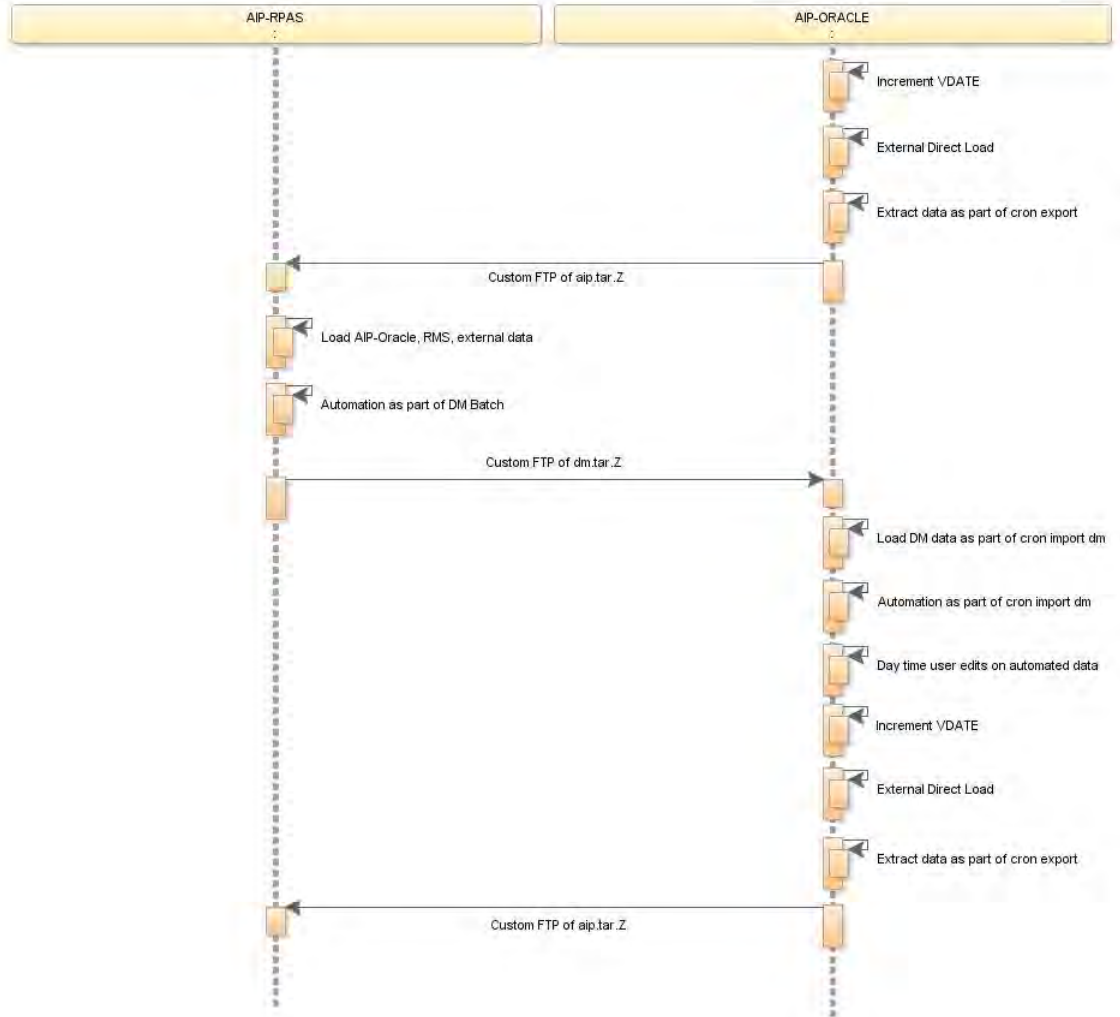
Figure 12-1 AIP-Oracle External Data Load interfaces
