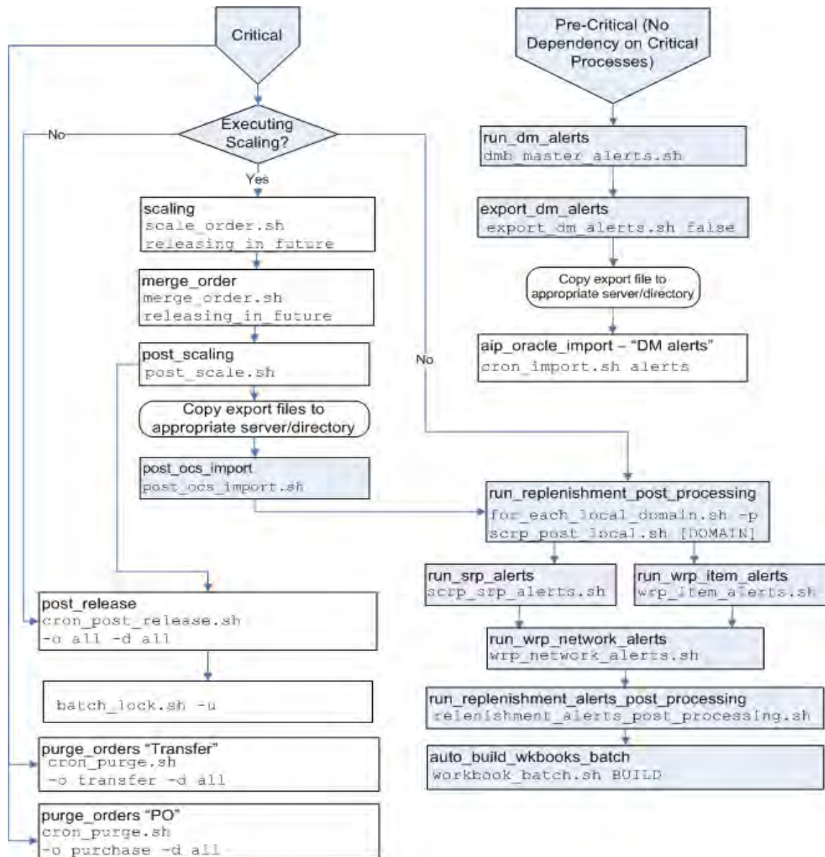
Figure 4-3 Post Critical Path Tasks Process Flow Diagram
