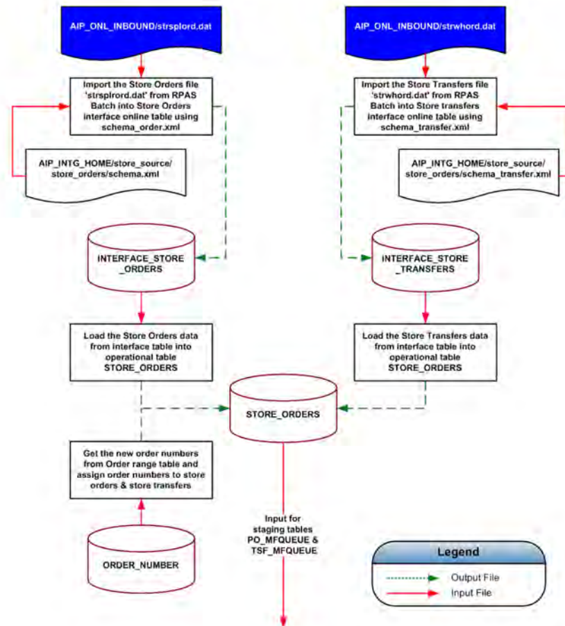
Figure 15-2 Store - Purchase Orders and Transfers Message Flow Diagram (1 of 2)
