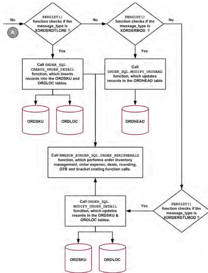
Figure 15-7 AIP Purchase Order Messages - RMS Load Process Diagram (2 of 2)
