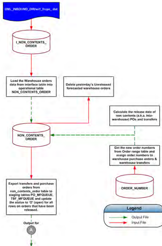
Figure 15-4 Warehouse - Purchase Orders and Transfers Message Flow Diagram (1 of 2)
