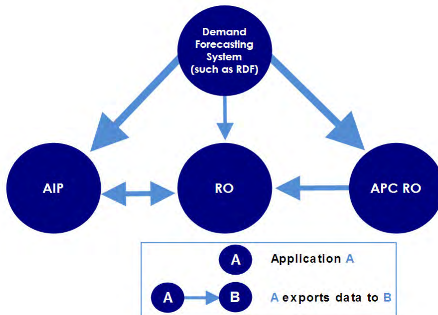
Figure 8–1 Integrated Inventory Planning Suite Conceptual Overview
