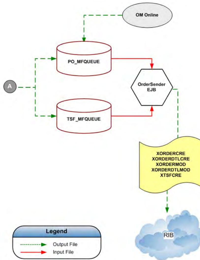
Figure 15-5 Warehouse - Purchase Orders and Transfers Message Flow (2 of 2)
