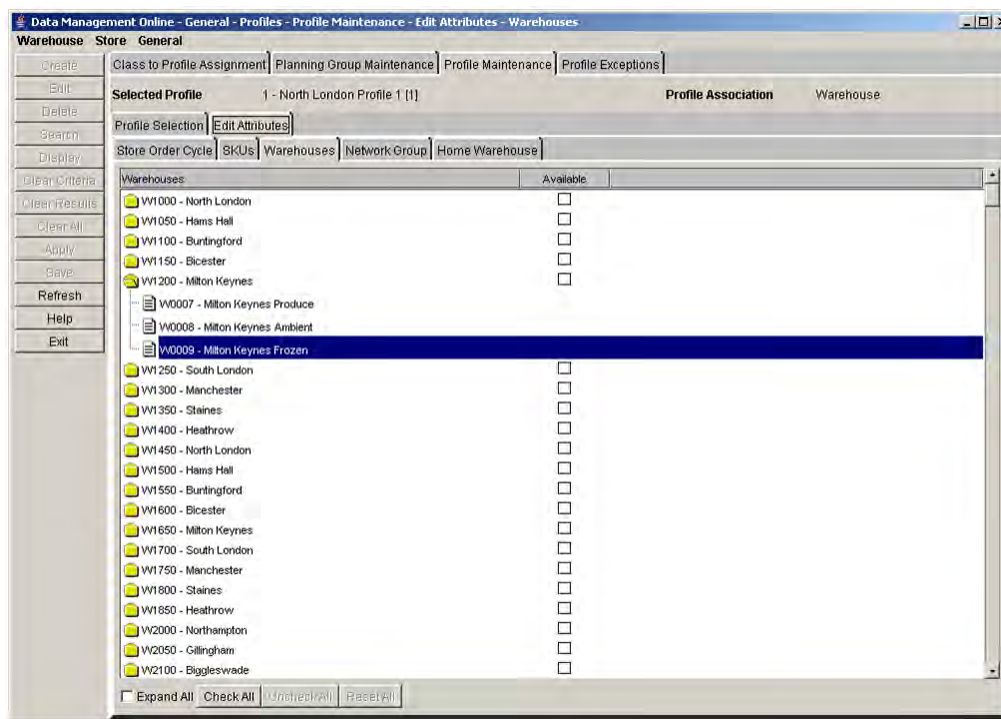
Figure 3-30 Warehouses Tab
