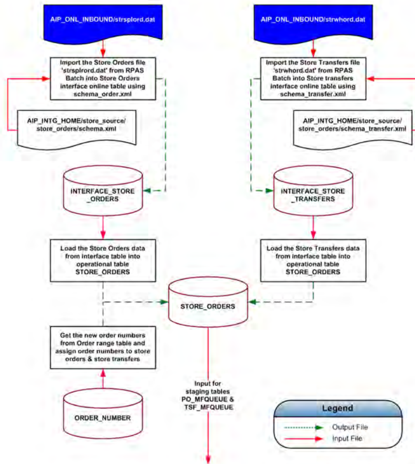
Figure 16-2 Store - Purchase Orders and Transfers Message Flow Diagram (1 of 2)
