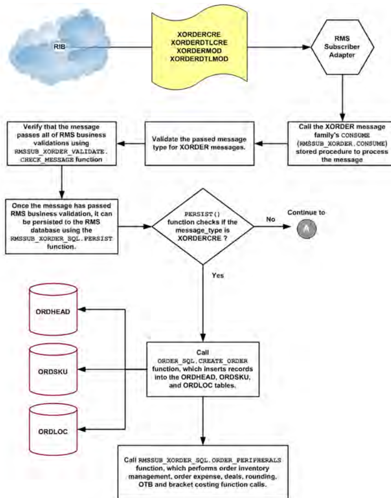
Figure 16–6 AIP Purchase Order Messages - RMS Load Process Diagram (1 of 2)
