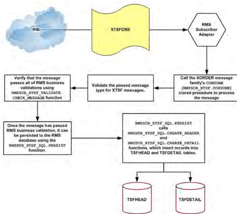
Figure 16–8 AIP Transfer Messages - RMS Load Process Diagram
