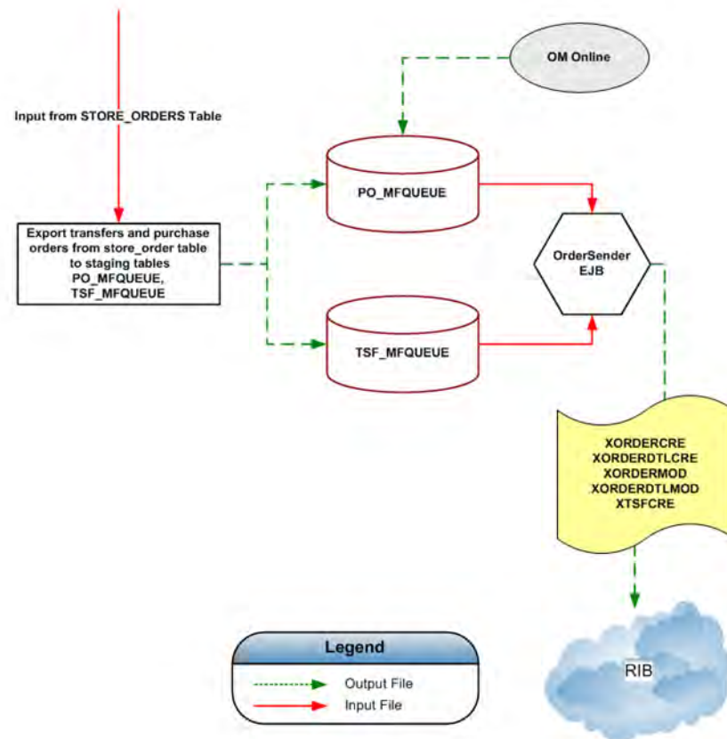
Figure 16–3 Store - Purchase Orders and Transfers Message Flow (2 of 2)
