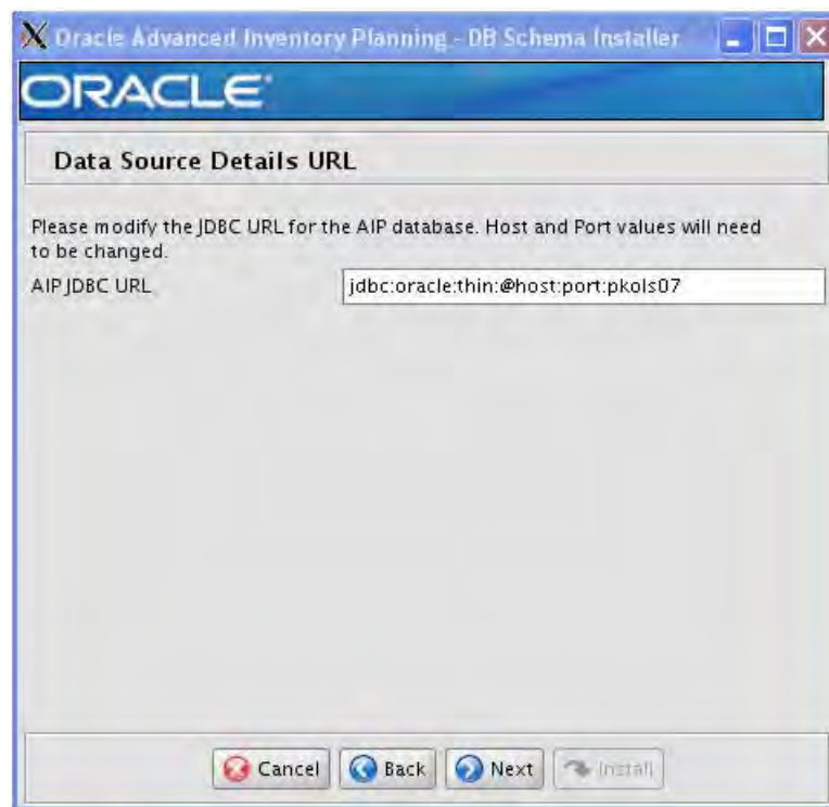
Figure 4–4 Data Source Details URL Window
