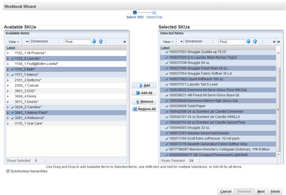
Figure 5–20 Workbook Wizard: Select SKU
