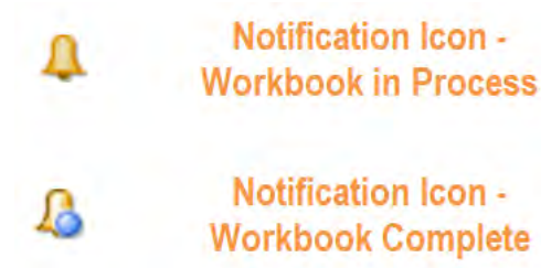
Figure 1-46 Notification Icons
