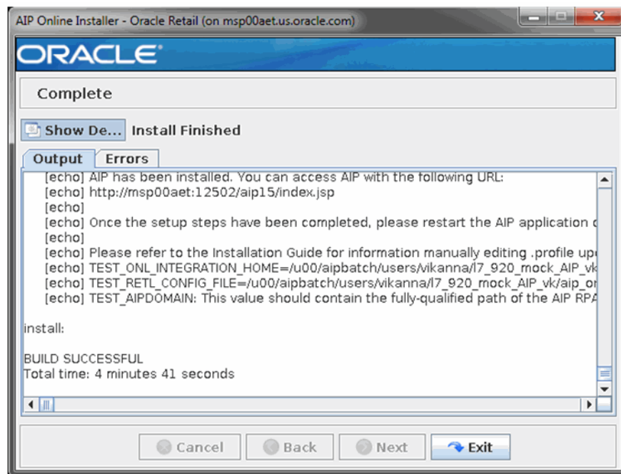
Figure 5–17 Complete Window
