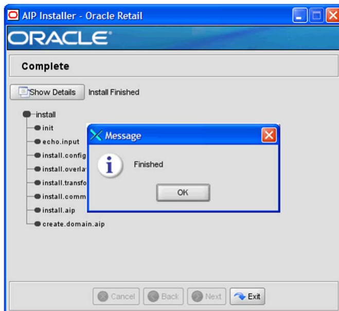
Figure 8–10 Complete Window
