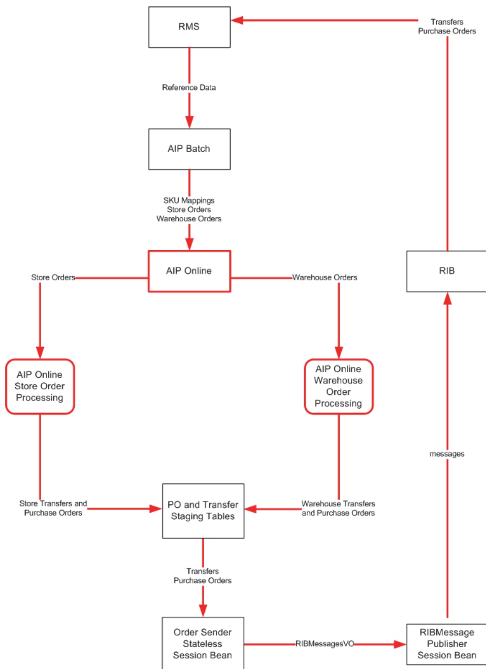
Figure 1–1 Data Flow
