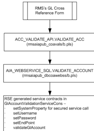
Figure 5–1 Process Flow for Web Service API
