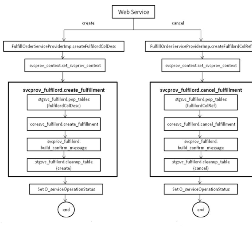
Figure 4–3 Web Service Deployment for Customer Order Fulfillment Requests
