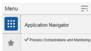
Figure 1–4 Application Navigator
