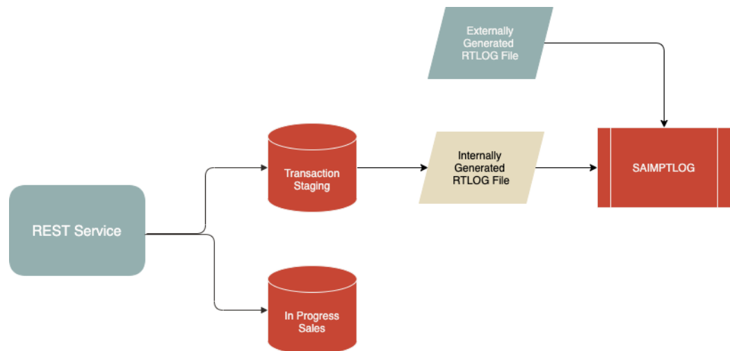
Figure 9–1 Importing Sales Data Process Flow
