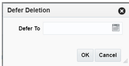
Figure 2–16 Defer Deletion
