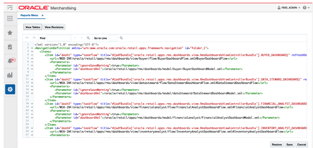
Figure 6–6 XML View
