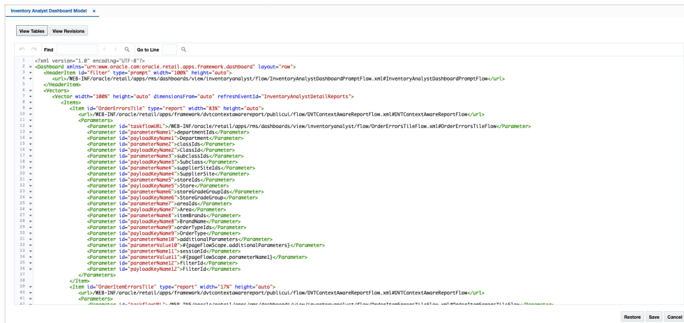
Figure 6–11 XML View
