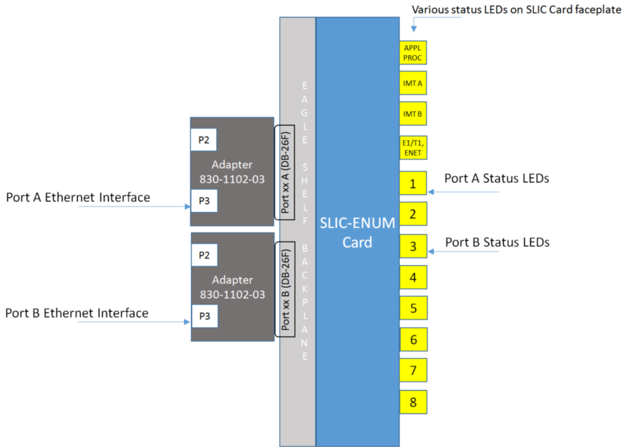
Figure 8: SLIC ENUM Card - Ethernet Interface Connections and Status LEDs
