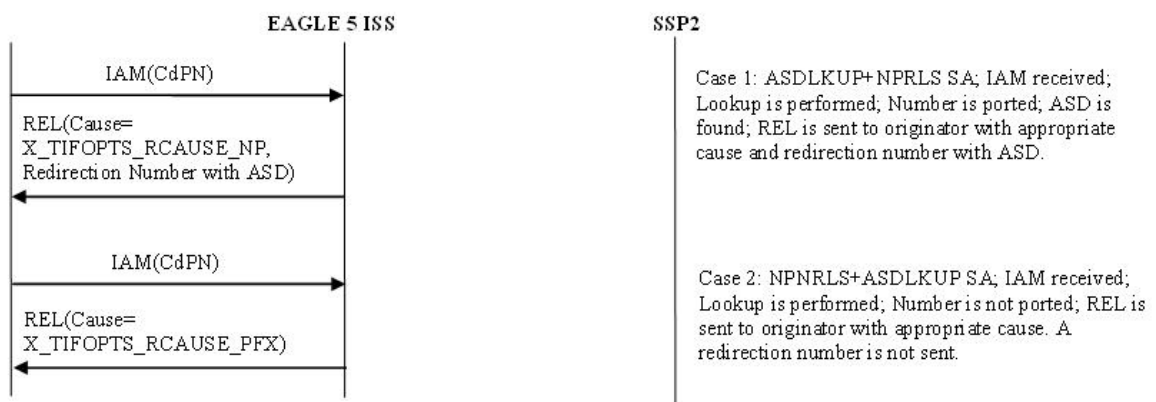
Figure 26: ISUP REL Message Flow for TIF ASD for TIF CdPN Service with NPRLS and NPNRLS SAs shows TIF ASD use cases with the NPRLS and NPNRLS Service Actions.
