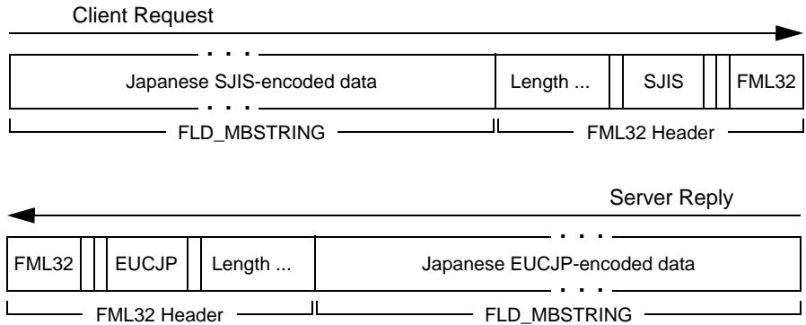
Figure 6-2 Using Global Encoding
