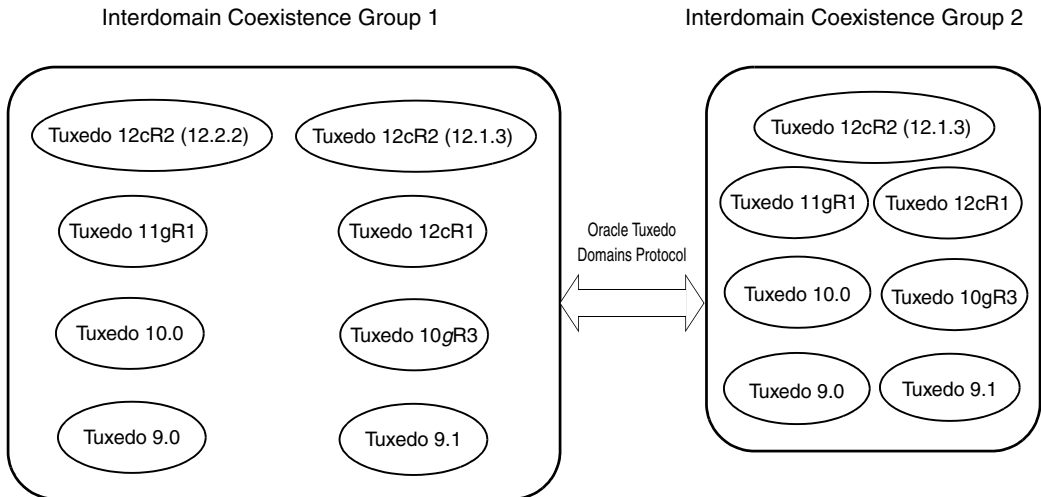
Figure 1-2 Interdomain Scenario 1
