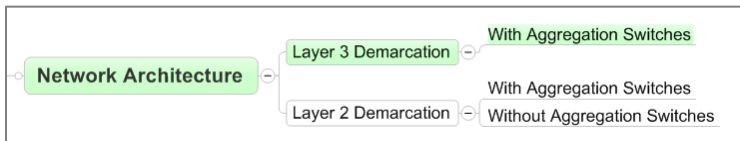
Figure 5: RMSNetwork Architecture*
