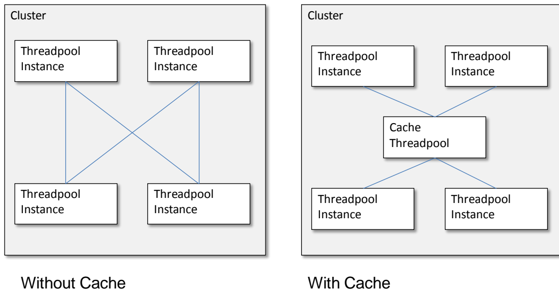
Figure 38 – Cache Architecture
