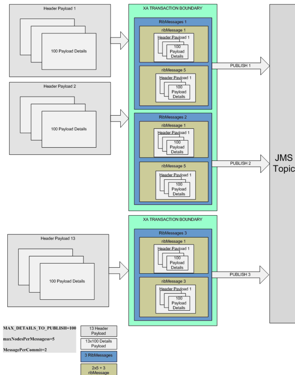
Figure 12–11 RIB Message Aggregation
