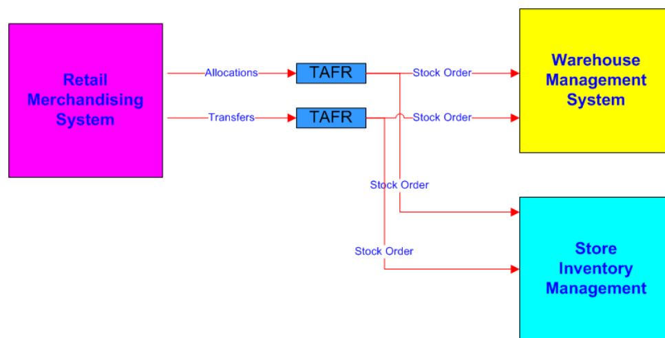
Figure 12–8 Logical View of the Oracle Retail Stock Order Flow
