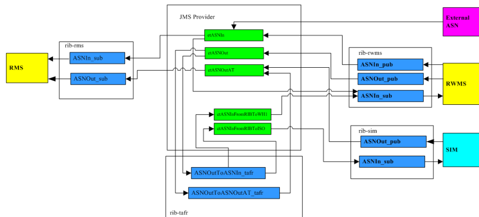
Figure 12–5 Functional Detailed View of the Oracle Retail ASNIn/ASNOOut Flows
