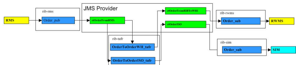
Figure 12–4 Functional Detailed View of the Oracle Retail Purchase Order Flow
