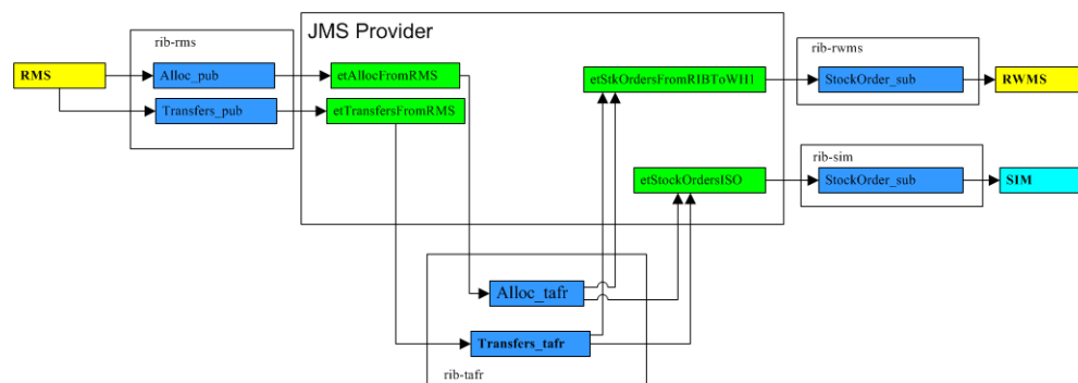
Figure 12–9 Functional Detail View of the Oracle Retail Stock Order Flow
