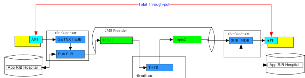
Figure 12–2 Generic Message Flow Diagram
