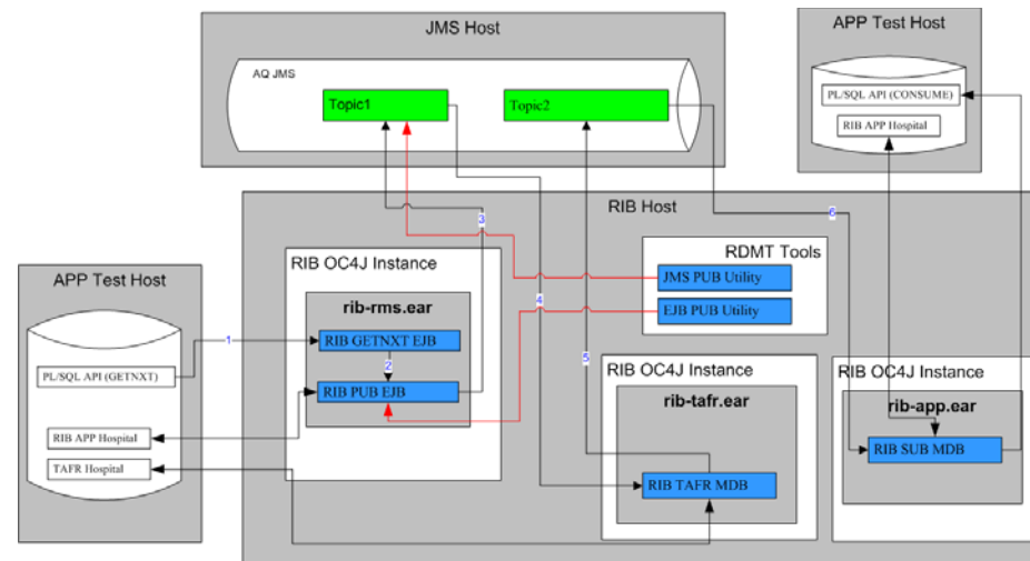
Figure 12–10 RIB Performance Test Harness
