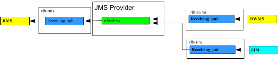
Figure 12–7 Functional Detail View of the Oracle Retail Receipts Flow
