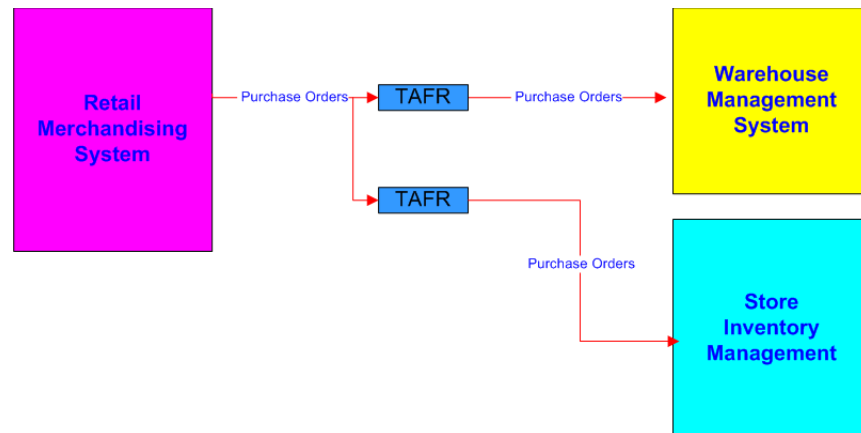
Figure 12–3 Logical View of the Oracle Retail Purchase Order Flow
