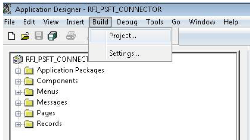
Figure 8–30 Project
