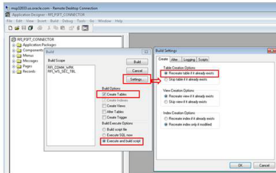
Figure 8-31 Build Settings
