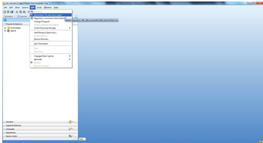
Figure 9–16 Disconnect
