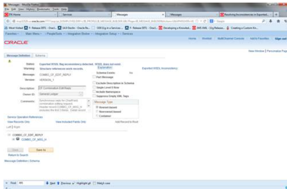
Figure 8-62 Service Admin
