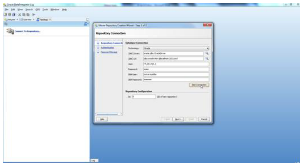
Figure 9–2 Repository Configuration
