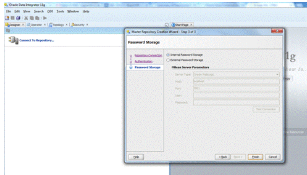
Figure 9–5 Password Storage
