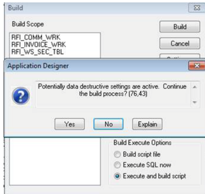
Figure 8–33 Build
