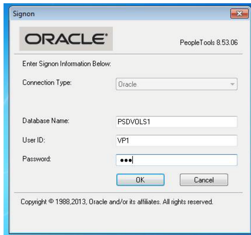
Figure 8–21 Signon
