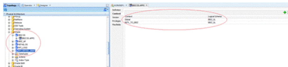
Figure 9–27 Verify
