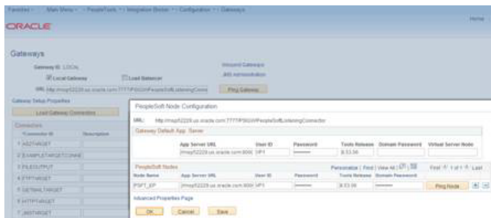
Figure 8–12 Ping Node
