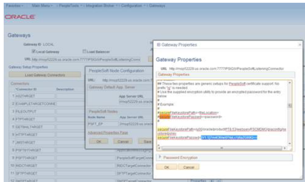
Figure 8–16 Password Encryption
