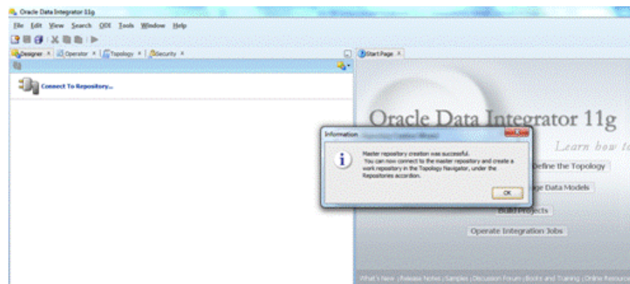
Figure 9–6 Information
