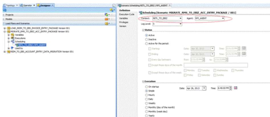
Figure 9–29 Scheduling
