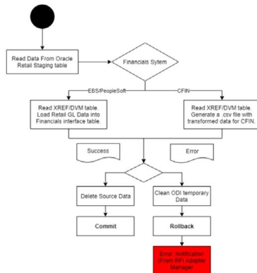
Figure 4-1 Accounting entries load process
