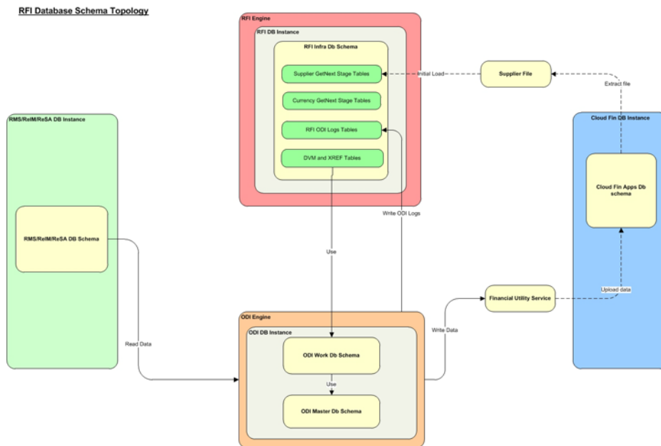
Figure 6–3 RFI Database Schema Topology for CFIN Integration
