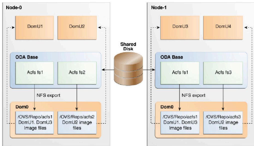
Figure 8-2 Architecture Overview of Oracle Database Appliance Virtualized Platform Shared Repositories
