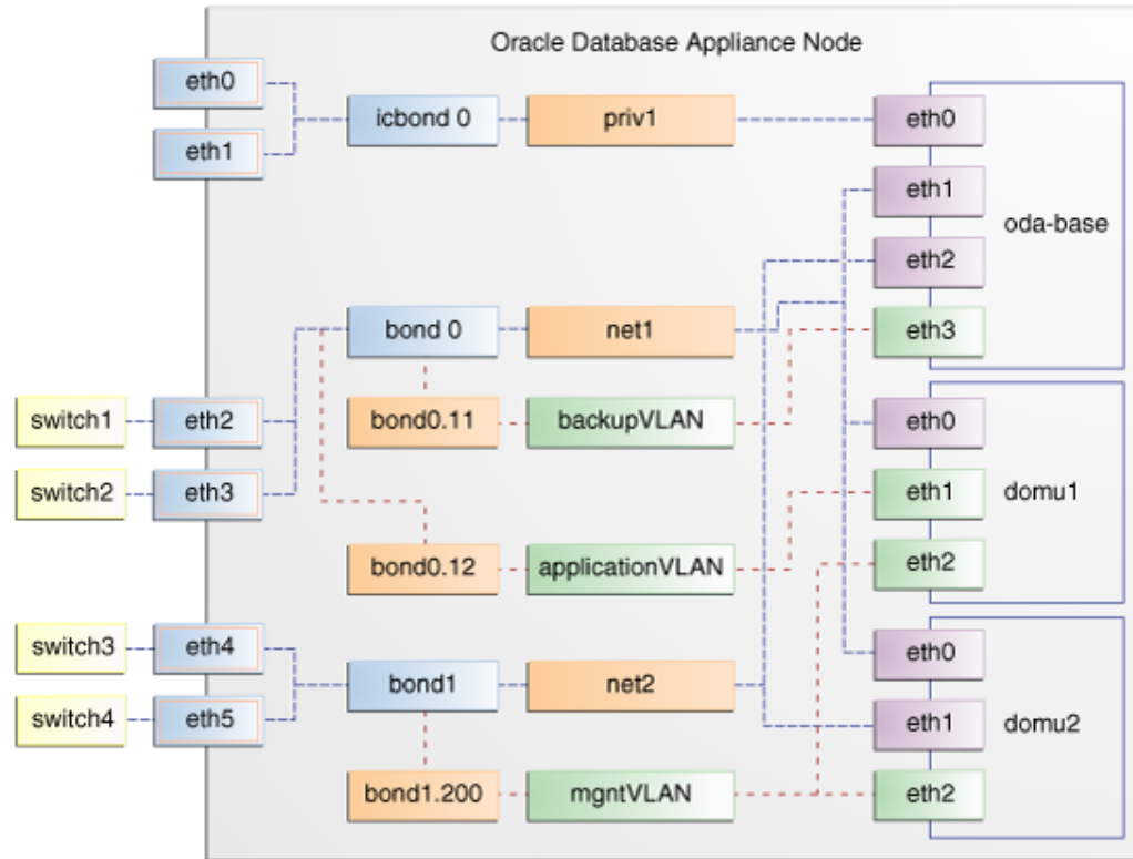
Figure 8-4 Oracle Database Appliance Virtualized Platform with Virtual Local Area Networks
