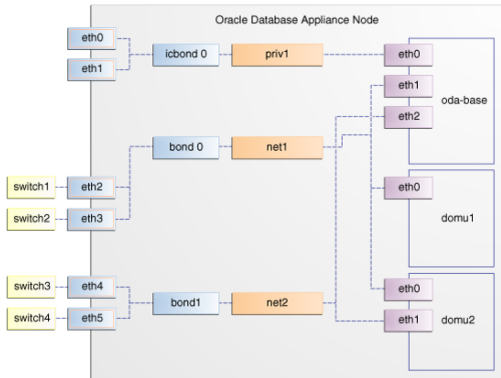
Figure 8-3 Basic Virtual Machine Local Area Network
