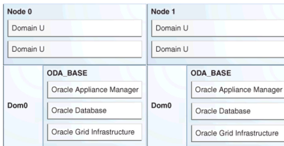
Figure 8-1 Oracle Database Appliance Virtualized Platform Architecture
