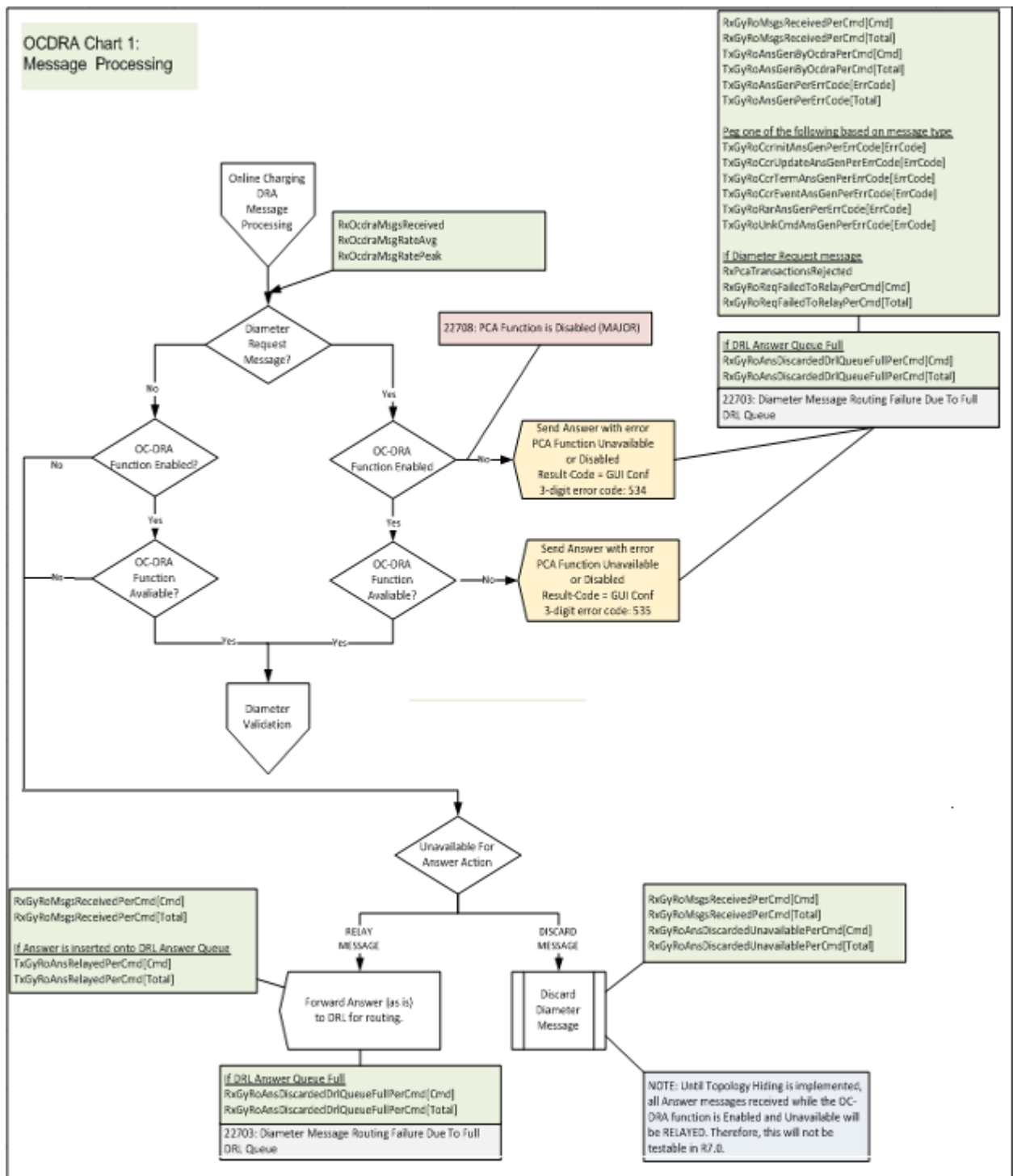
Figure 71: Message Processing
