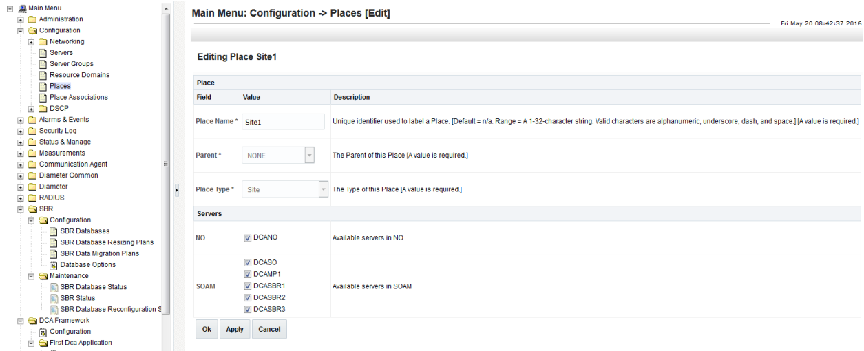
Figure 23: Places Configuration
