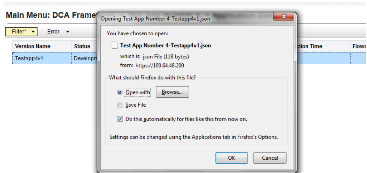
Figure 57: NO Export
