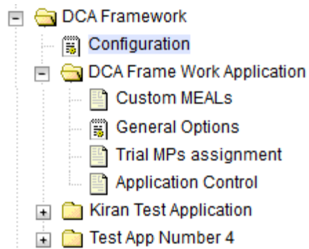
Figure 45: NO Screens
