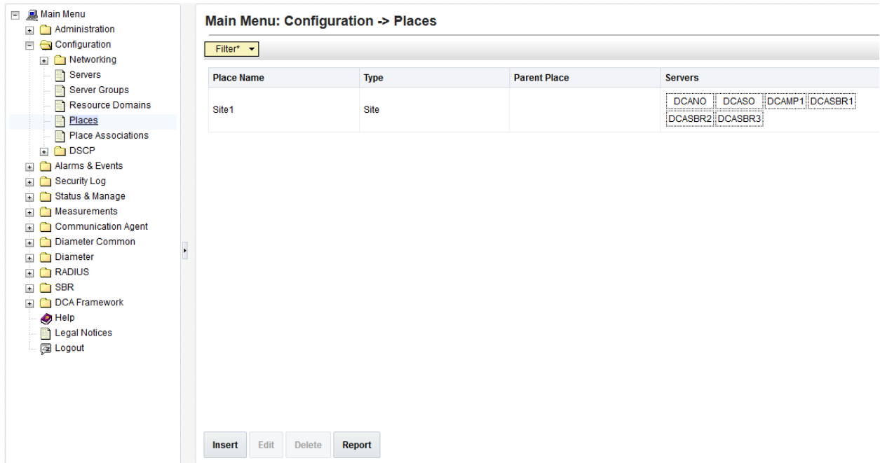
Figure 24: View Places
