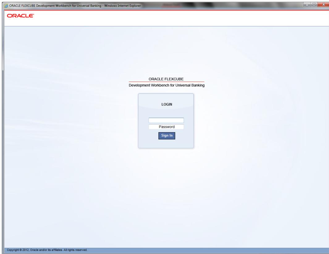
Fig 3.1: Login Screen
