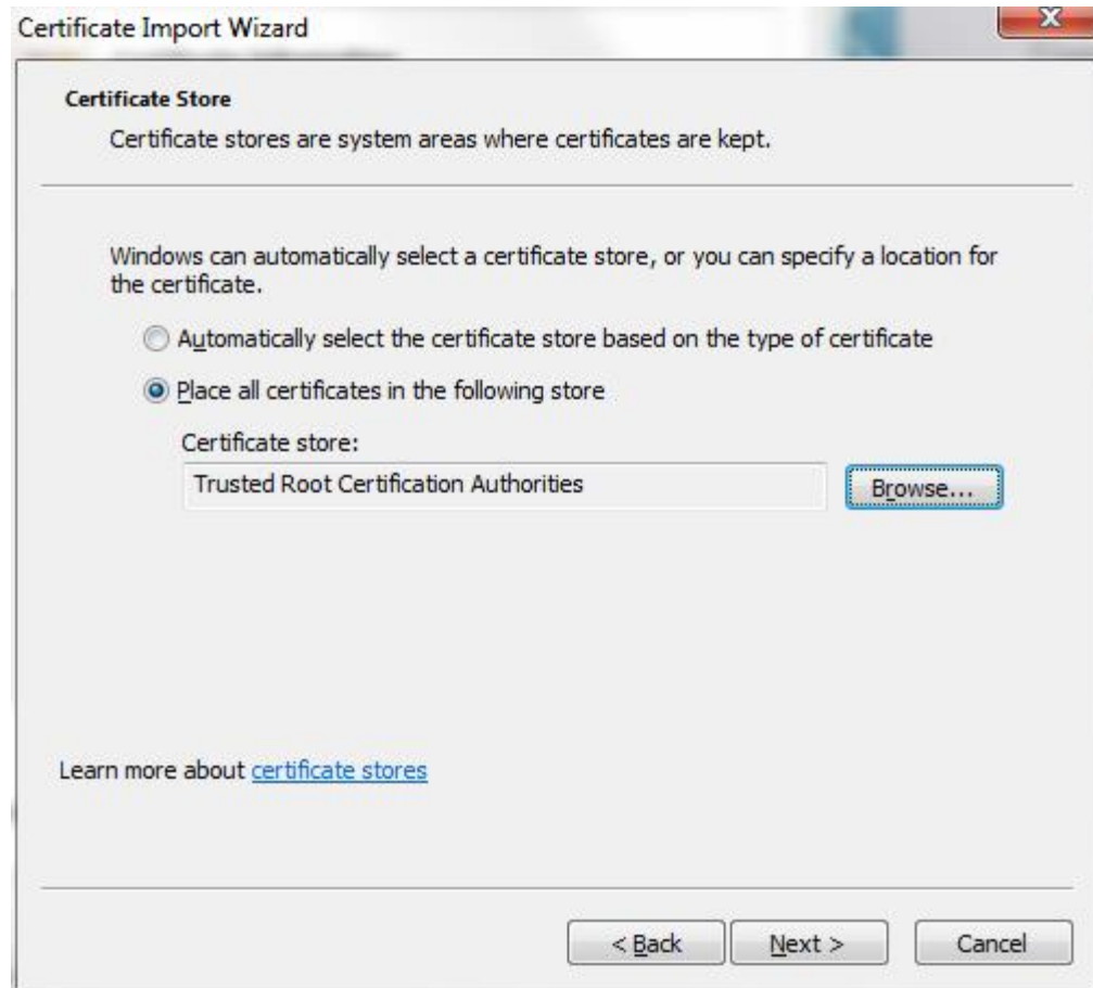
Figure 3-15 Certificate Store
