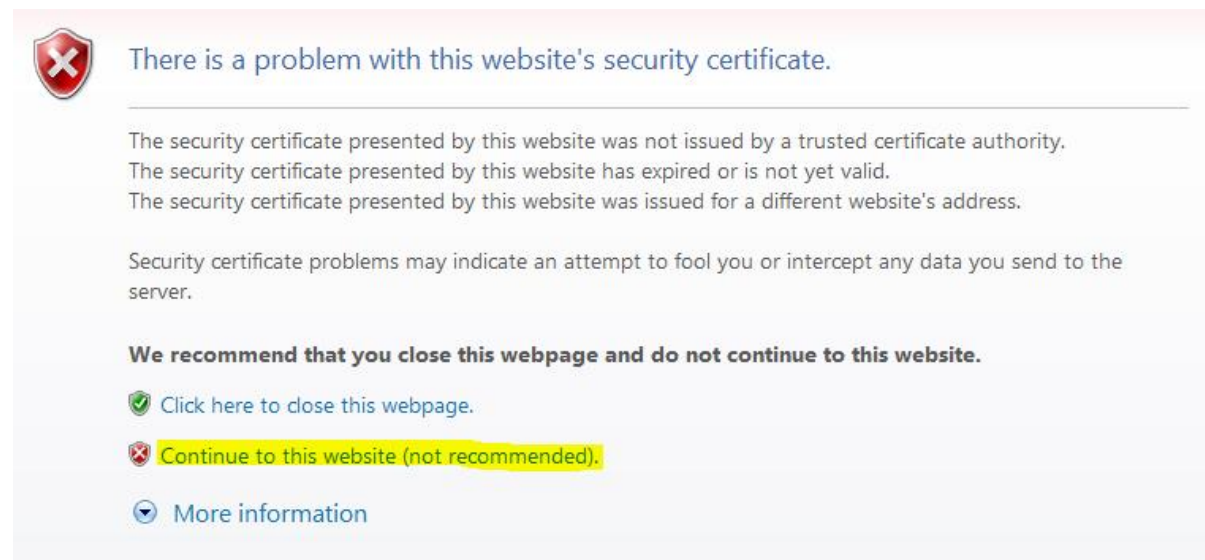
Figure 3-8 Security Certificate
