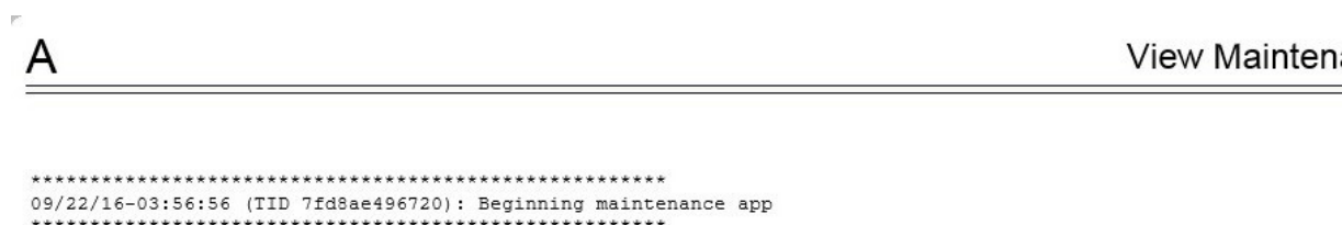
Figure 3-61 Log Viewer
