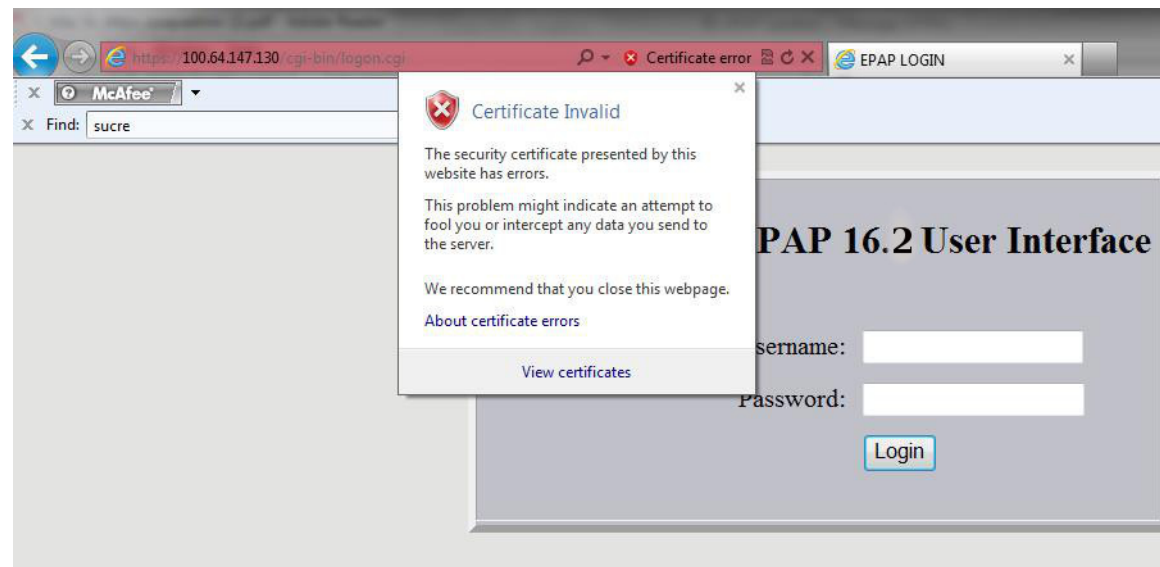
Figure 3-10 Certificate Error
