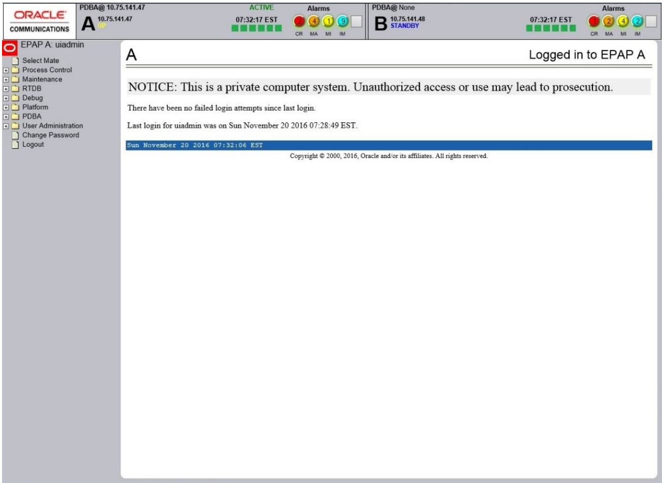
Figure 3-22 EPAP GUI
