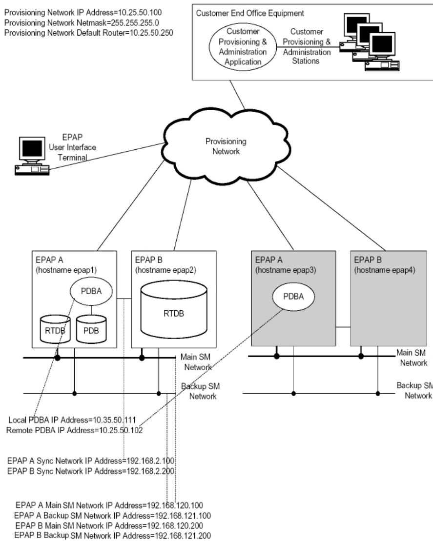
Figure 1: Example EPAP/PDBA Network
