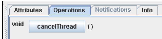
Figure 47: CancelThread Example
