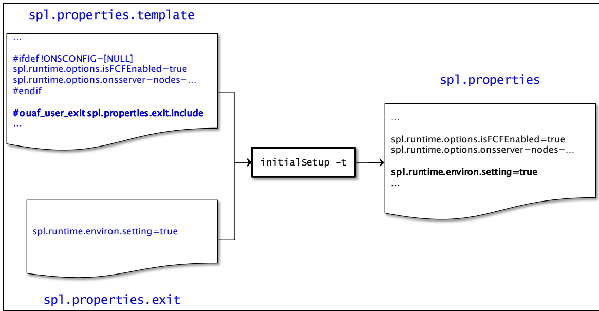
Figure 40: Include Files
