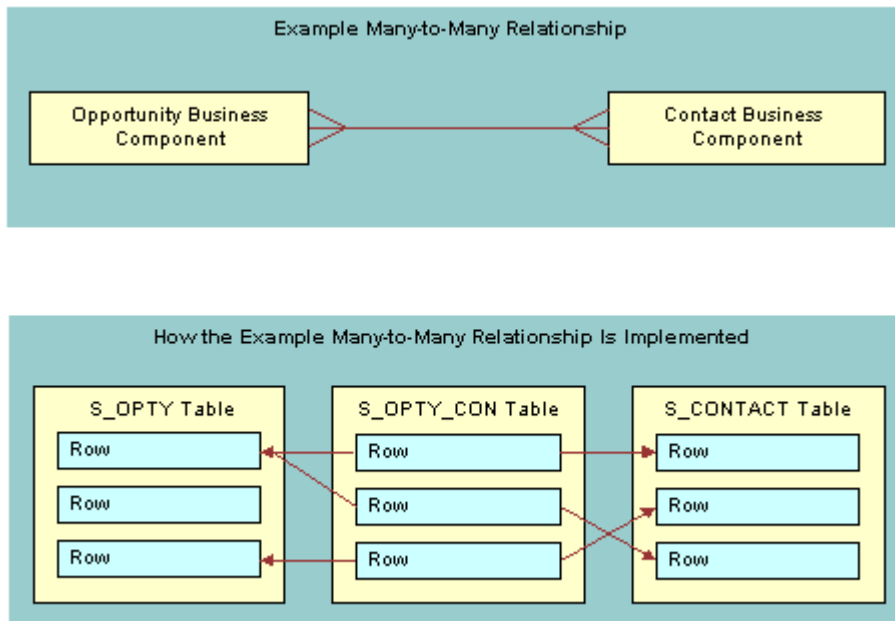
Figure 81. Example Many-to-many Relationship Between Two Business Components
