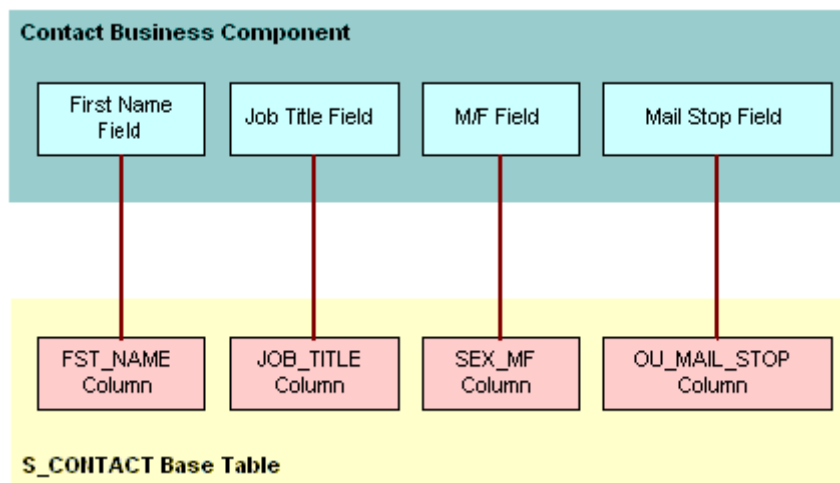
Figure 10. Example of How Fields in a Business Component Reference Columns in a Base Table
