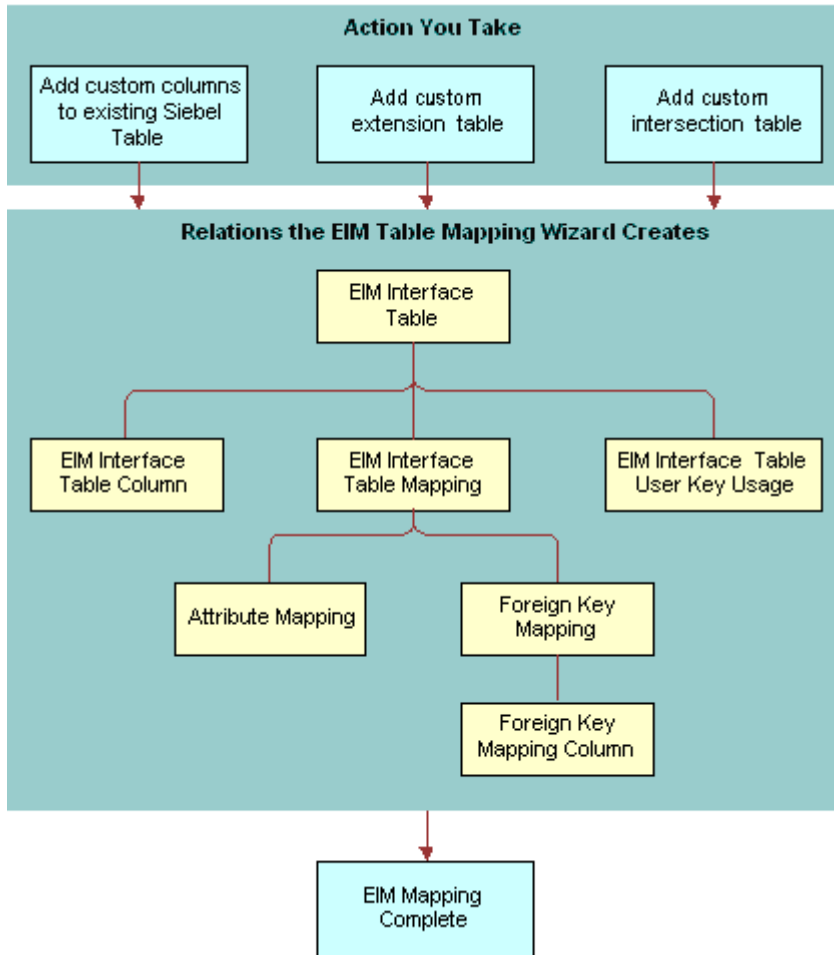
Figure 92. Relations That the EIM Table Mapping Wizard Creates
