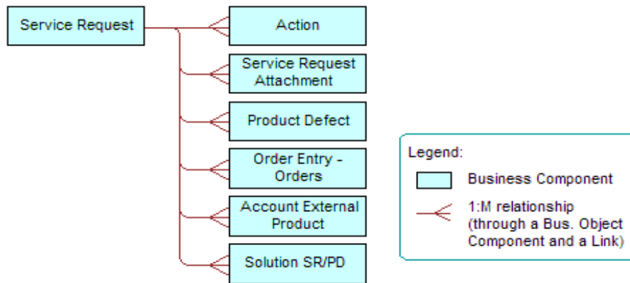
Figure 68. Relationships and Objects in the Service Request Business Object That Siebel CRM Uses in the Service Request Explorer View
