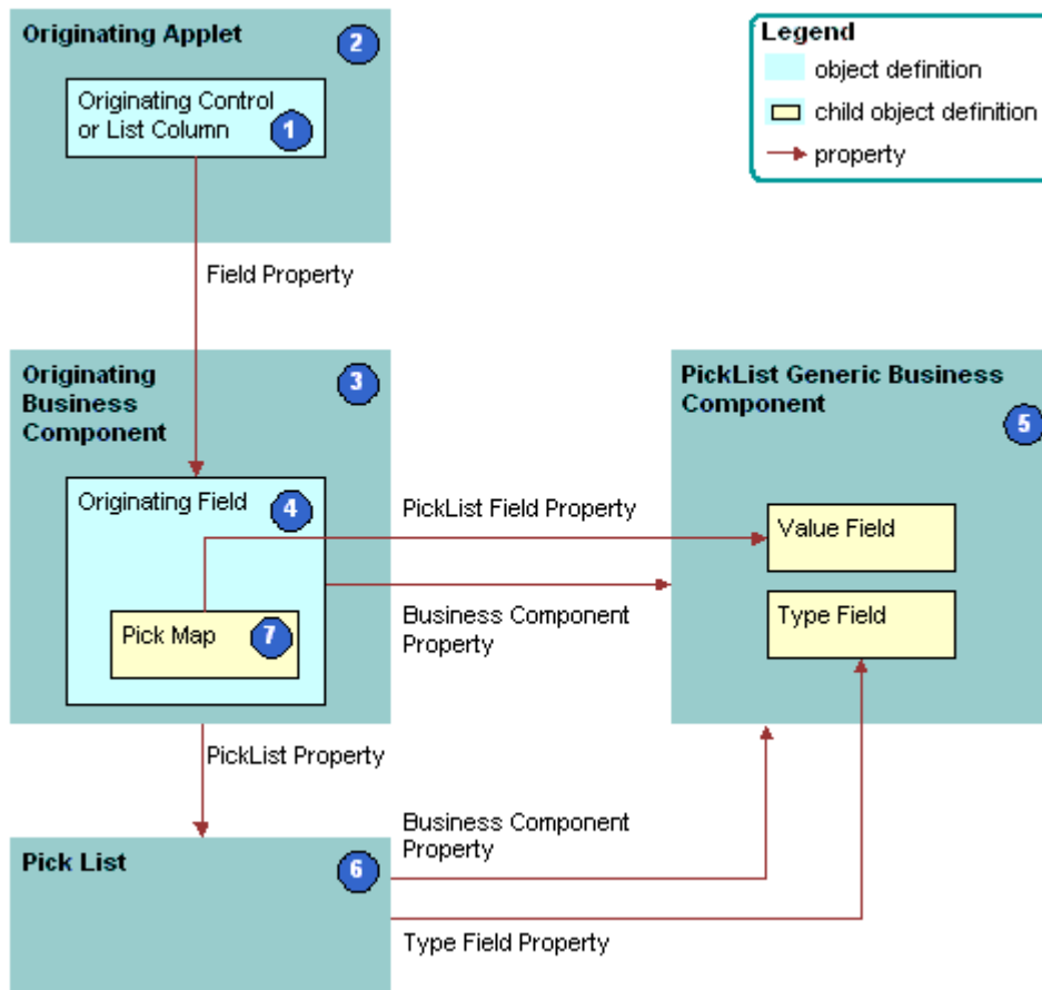
Figure 70. How Siebel CRM Creates a Static List
