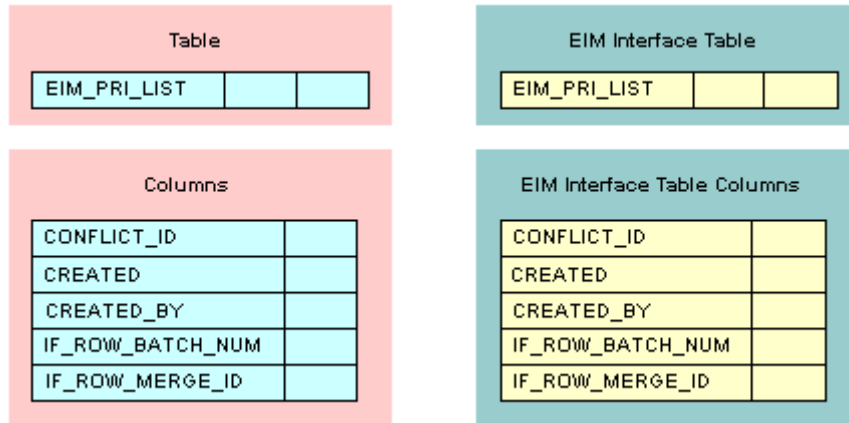
Figure 88. Child Columns of an Interface Table Are the Same as Child Columns of a Table
