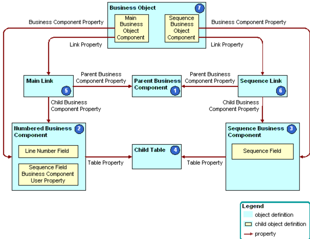
Figure 16. How Siebel CRM Creates a Sequence Field
