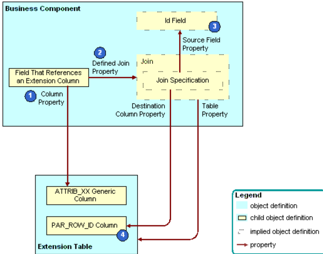
Figure 6. How Siebel CRM Creates an Explicit Join
