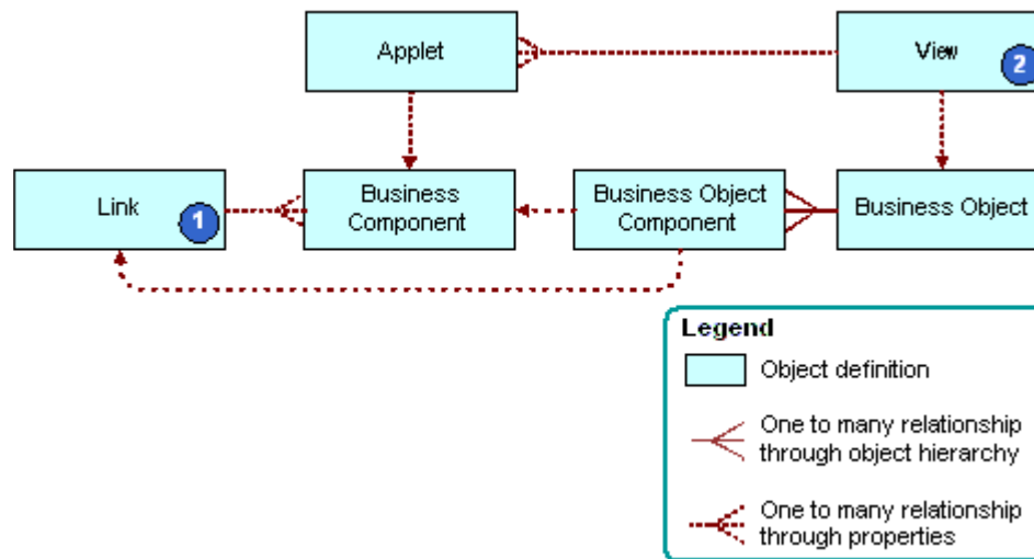
Figure 23. How a Business Object Uses a Link
