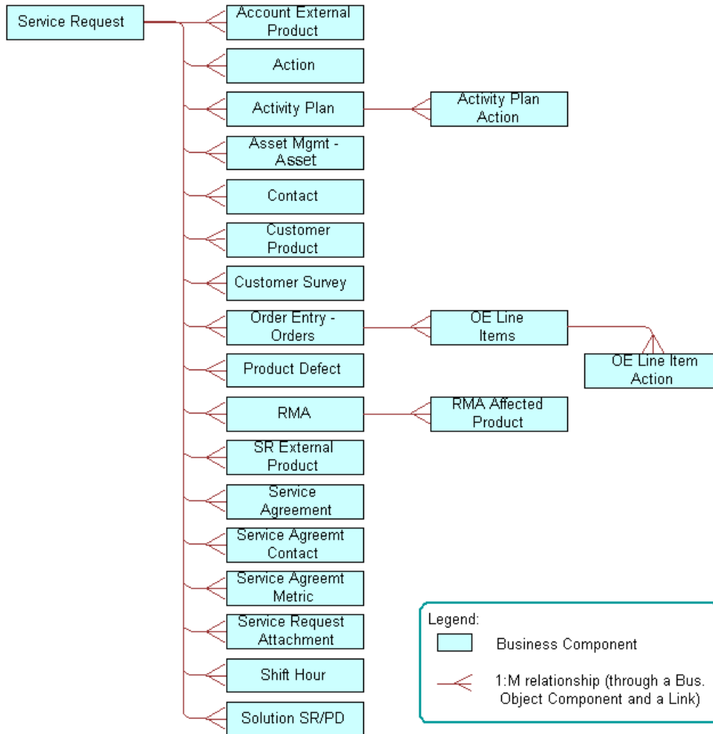
Figure 67. Relationships and Objects in the Service Request Business Object
