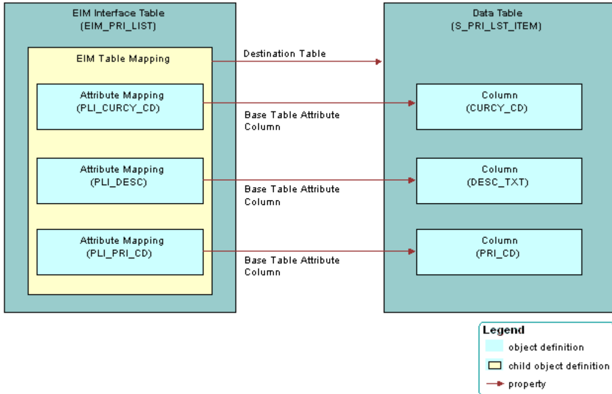
Figure 90. Example of How an EIM Table Mapping References a Data Table
