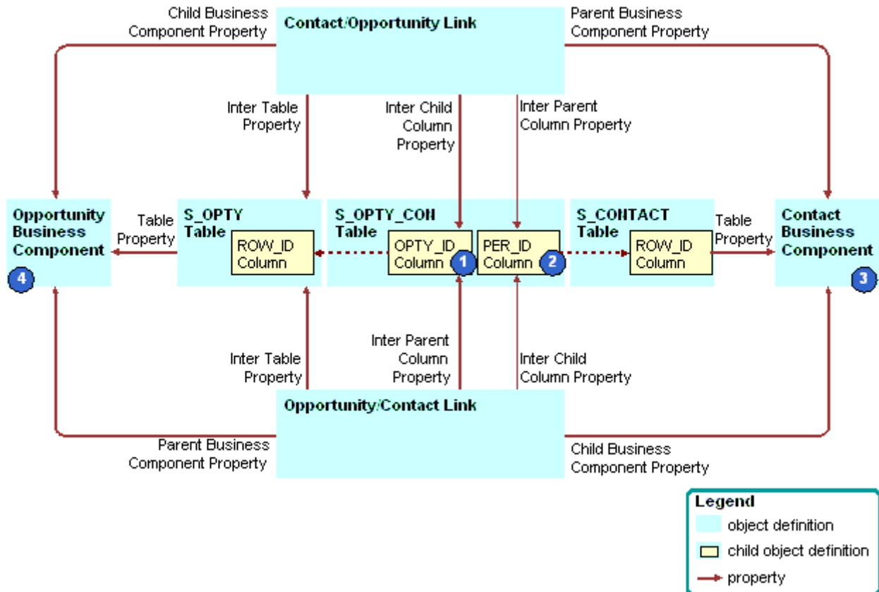
Figure 9. Example of How Siebel CRM Creates a Many-To-Many Relationship
