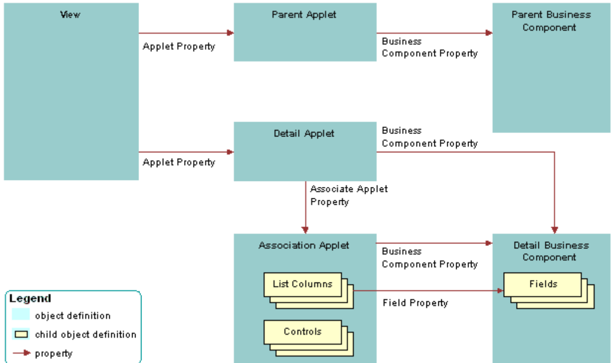
Figure 83. Generic Picture of How Siebel CRM Creates an Association Applet
