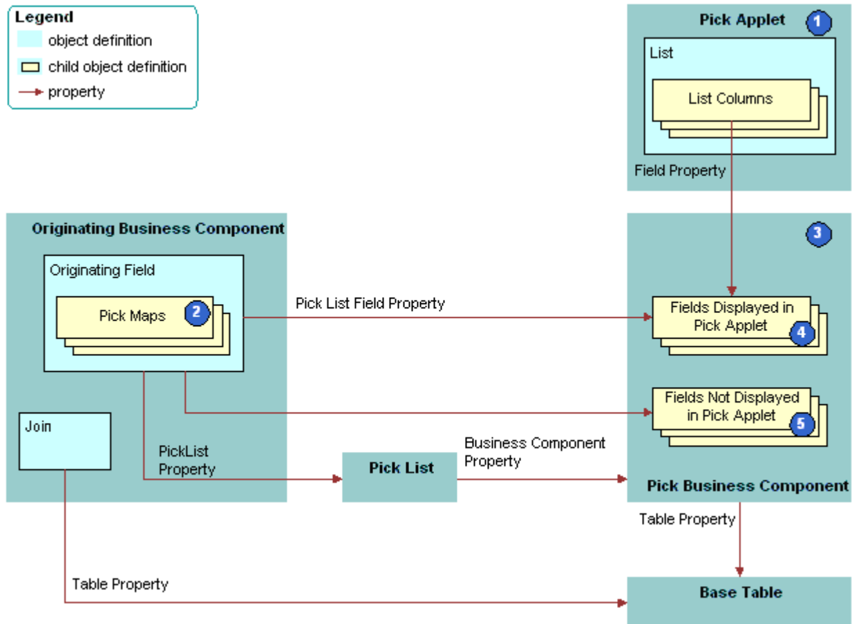
Figure 78. How Siebel CRM Constrains a Dynamic List
