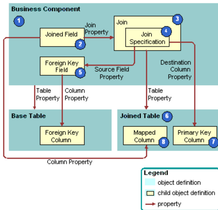
Figure 18. How Siebel CRM Creates a Join
