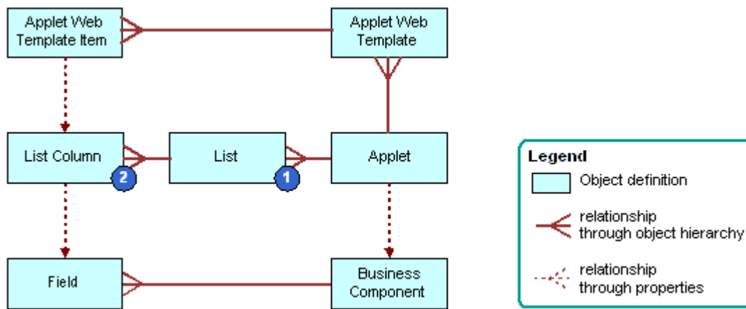
Figure 31. How Siebel CRM Creates a List Applet
