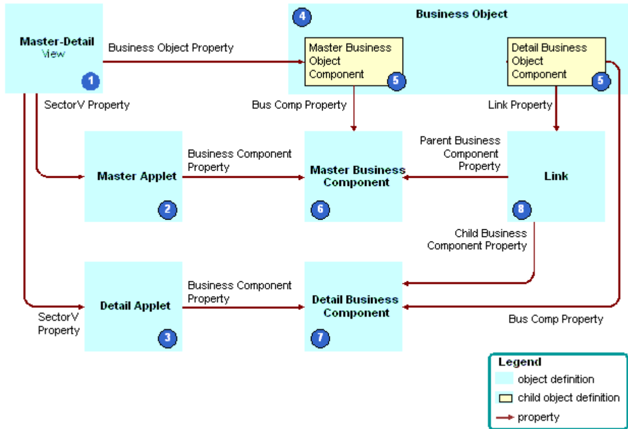
Figure 33. How Siebel CRM Creates a Master-Detail View
