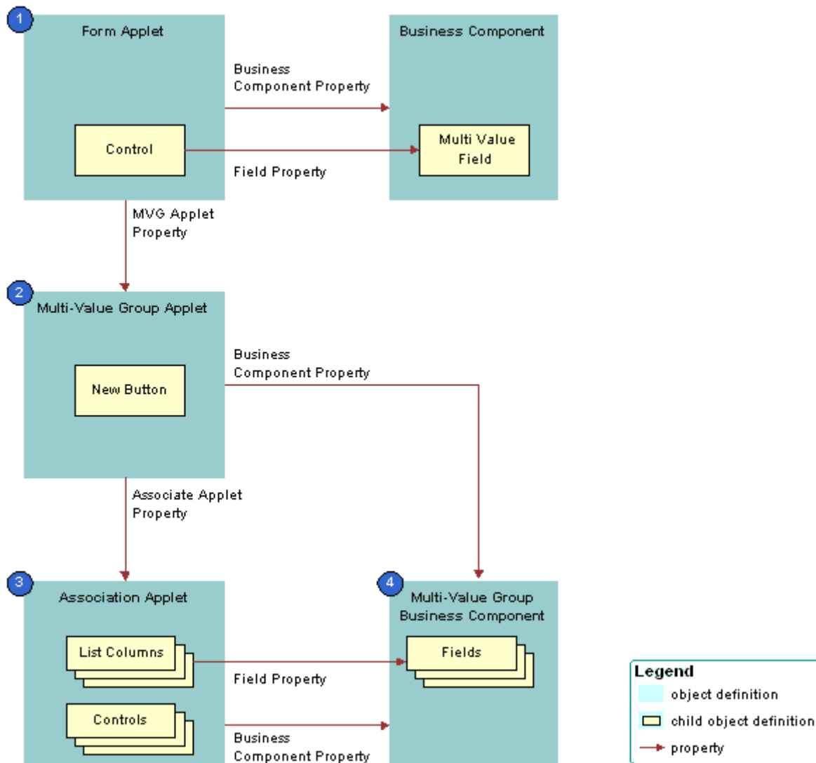
Figure 85. How Siebel CRM Creates an Association Applet It Calls from a Multi-Value Group Applet
