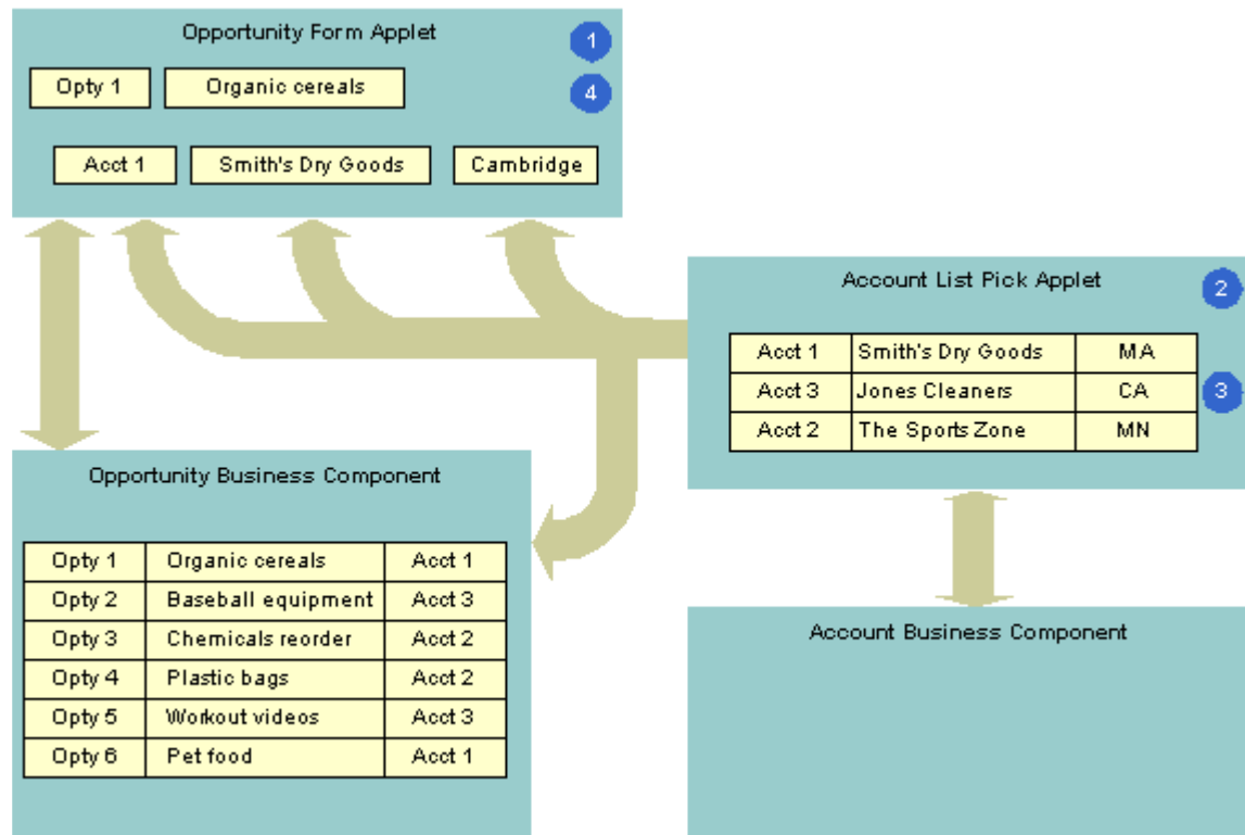
Figure 73. Example of How Data Flows in a Pick Applet
