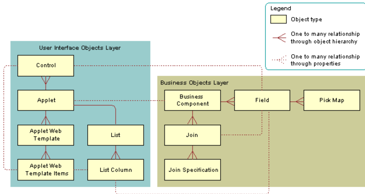
Figure 74. Relationships Between Object Types That Siebel CRM Uses to Create a Dynamic List
