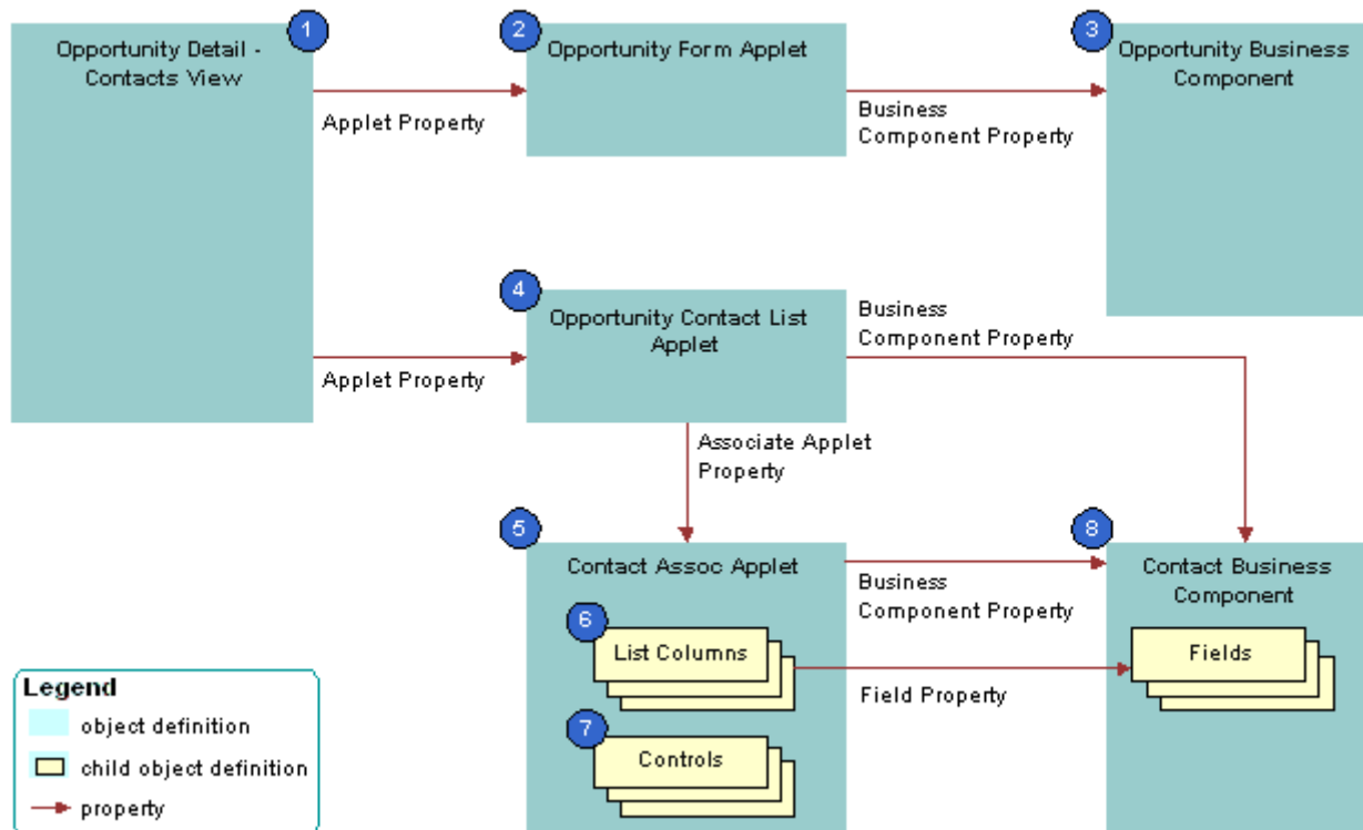
Figure 84. Example of How Siebel CRM Creates an Association Applet
