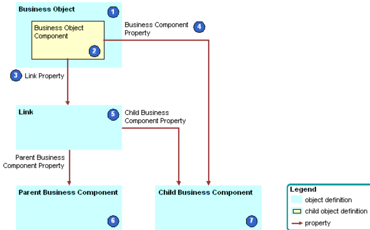
Figure 29. How Siebel CRM Creates a Business Object
