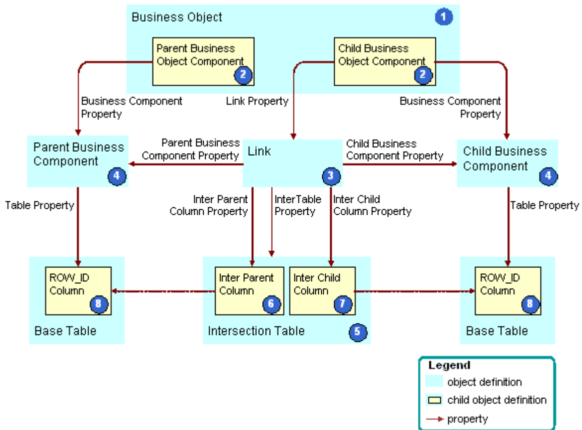
Figure 8. How Siebel CRM Creates an Intersection
