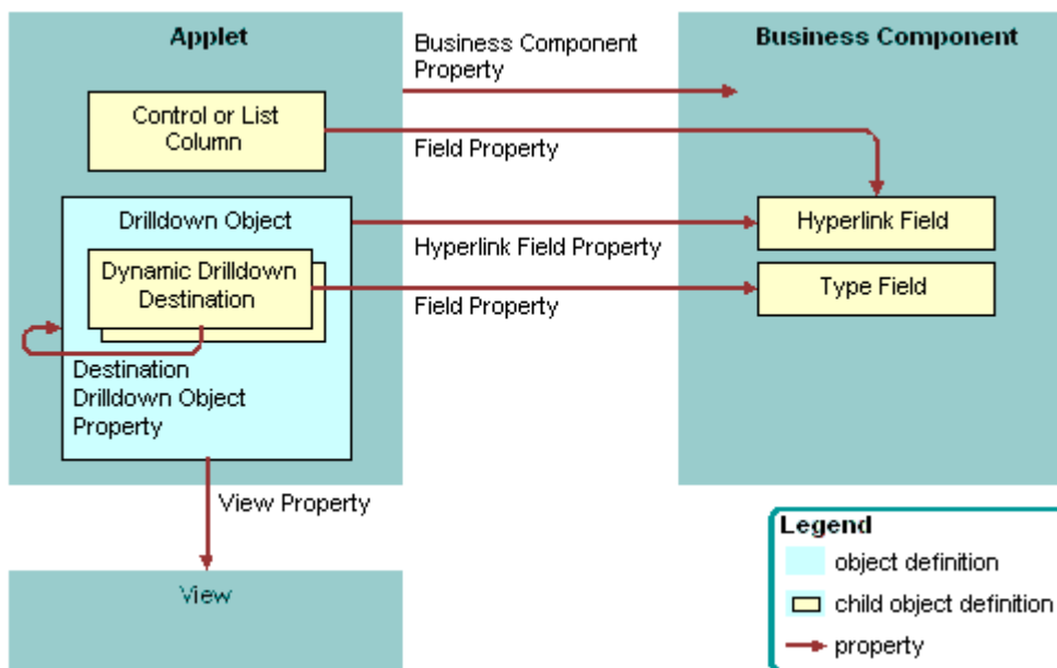
Figure 35. How Siebel CRM Creates a Dynamic Drilldown
