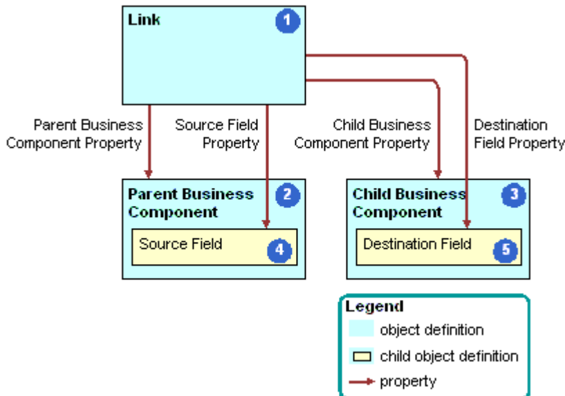
Figure 21. Objects and Relationships in a Link
