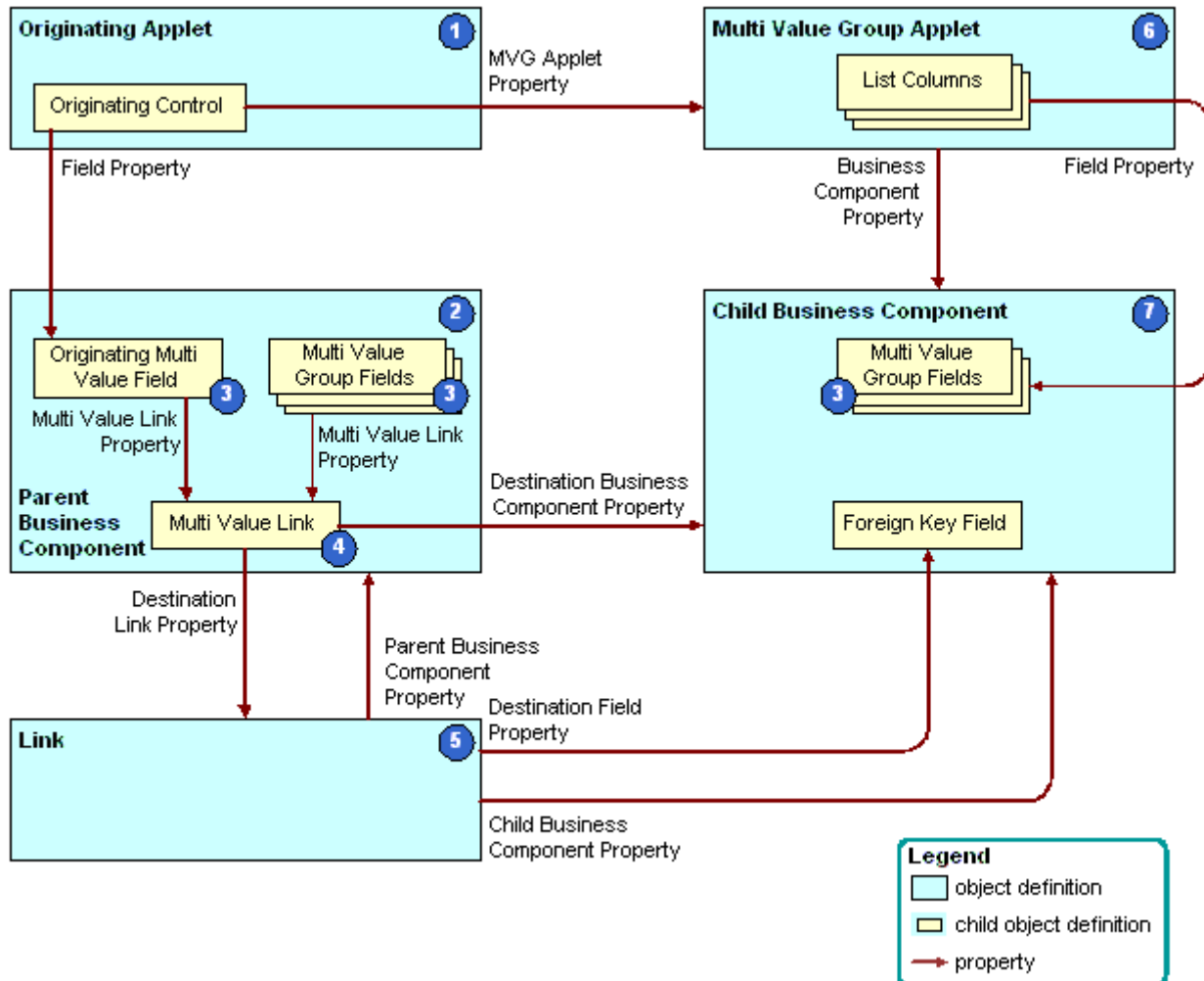
Figure 80. Objects and Properties Siebel CRM Uses to Create a Multi-Value Group Applet
