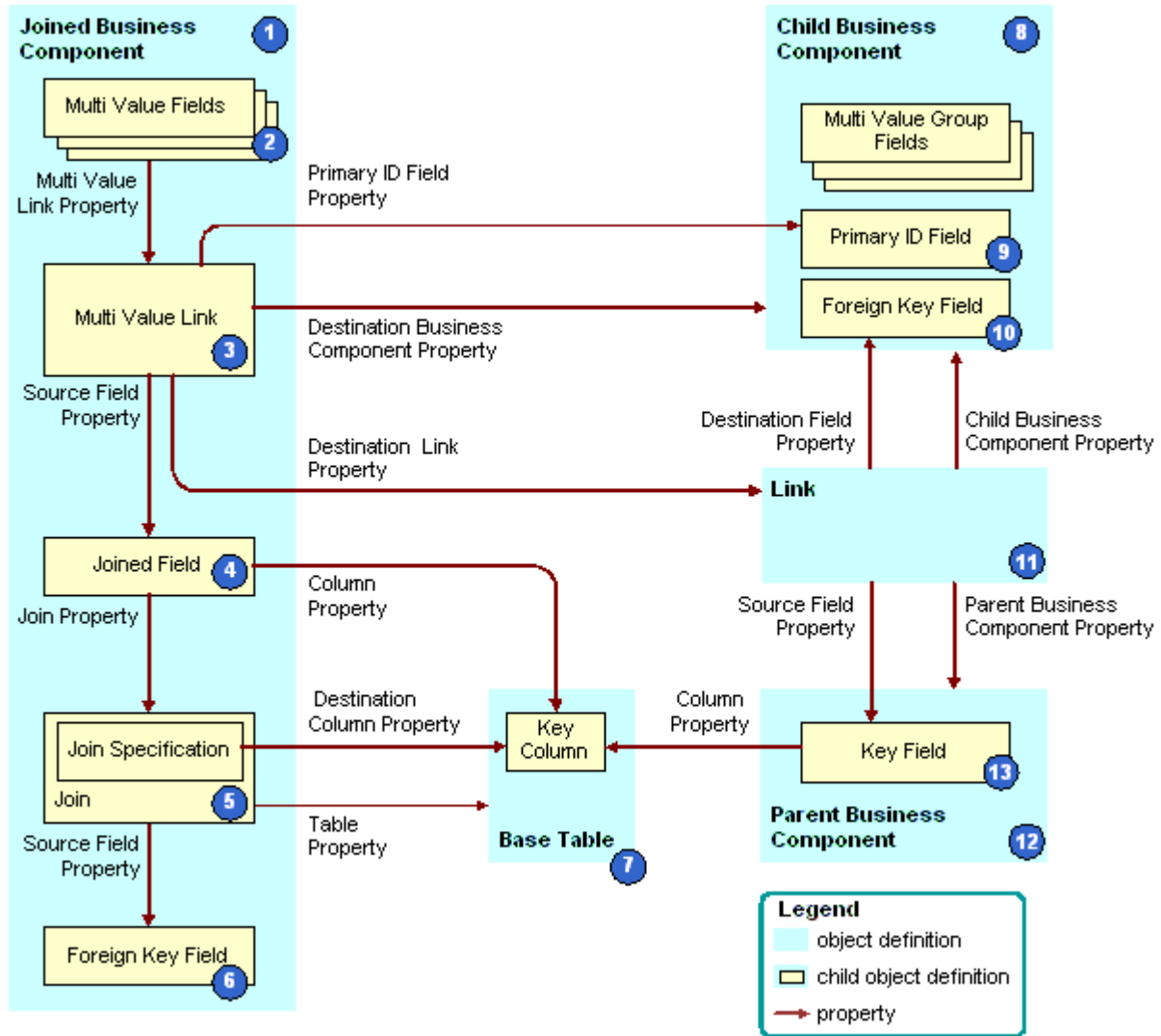
Figure 22. How Siebel CRM Creates an Indirect Multi-Value Link
