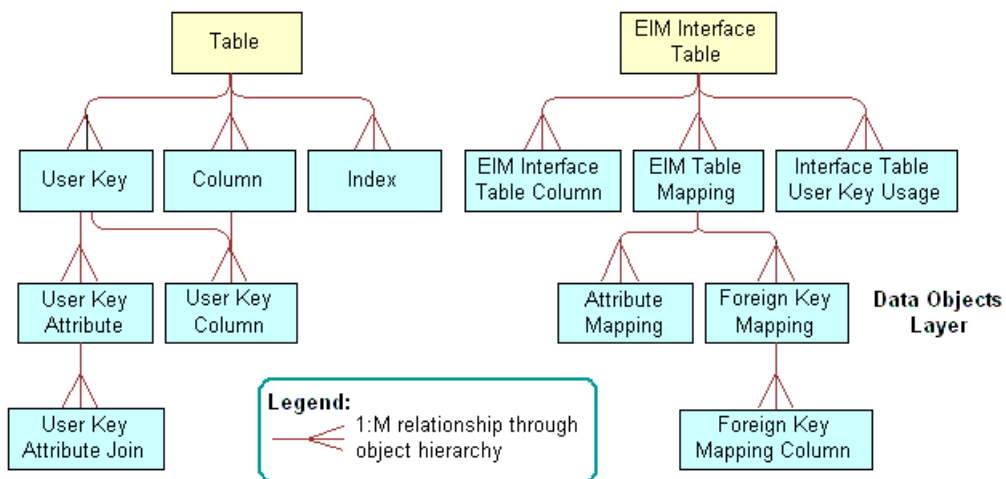
Figure 87. Objects and Relationships That EIM Uses
