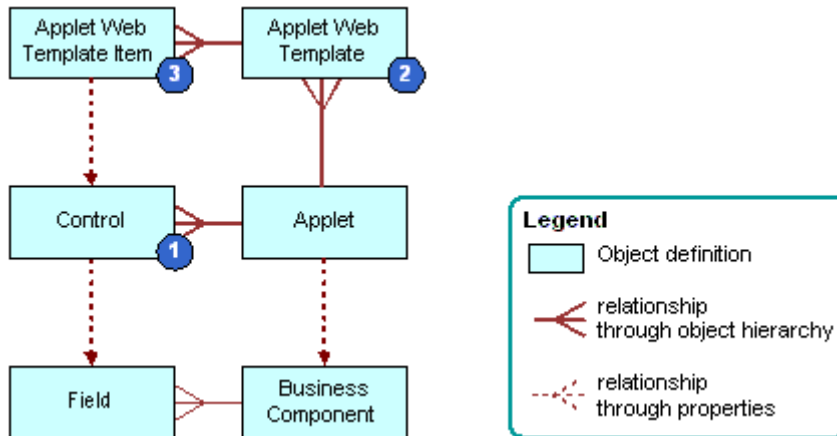
Figure 30. How Siebel CRM Creates a Form Applet
