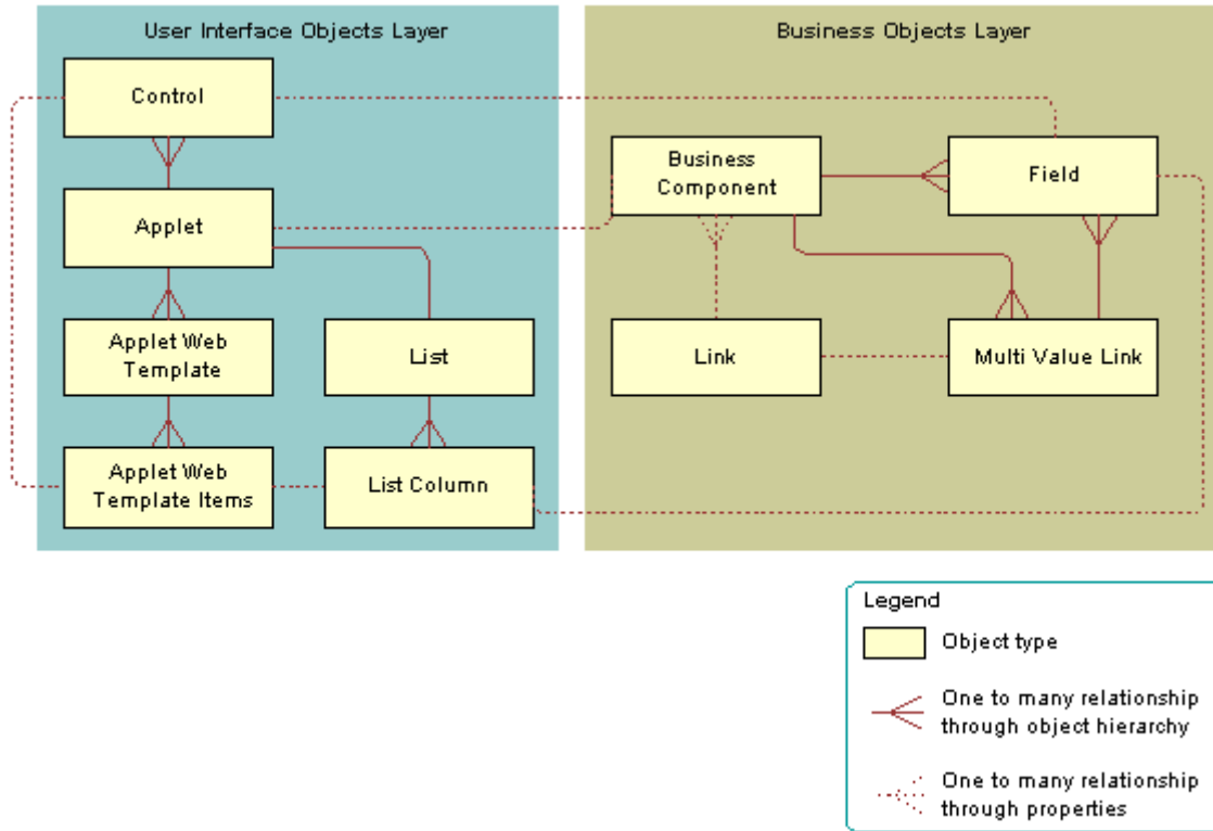
Figure 79. Relationships and Objects That Siebel CRM Uses in a View Multi-Value Group Applet
