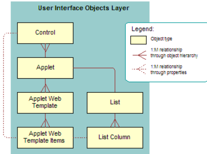
Figure 82. Relationships and Objects That Siebel CRM Uses to Create an Association Applet
