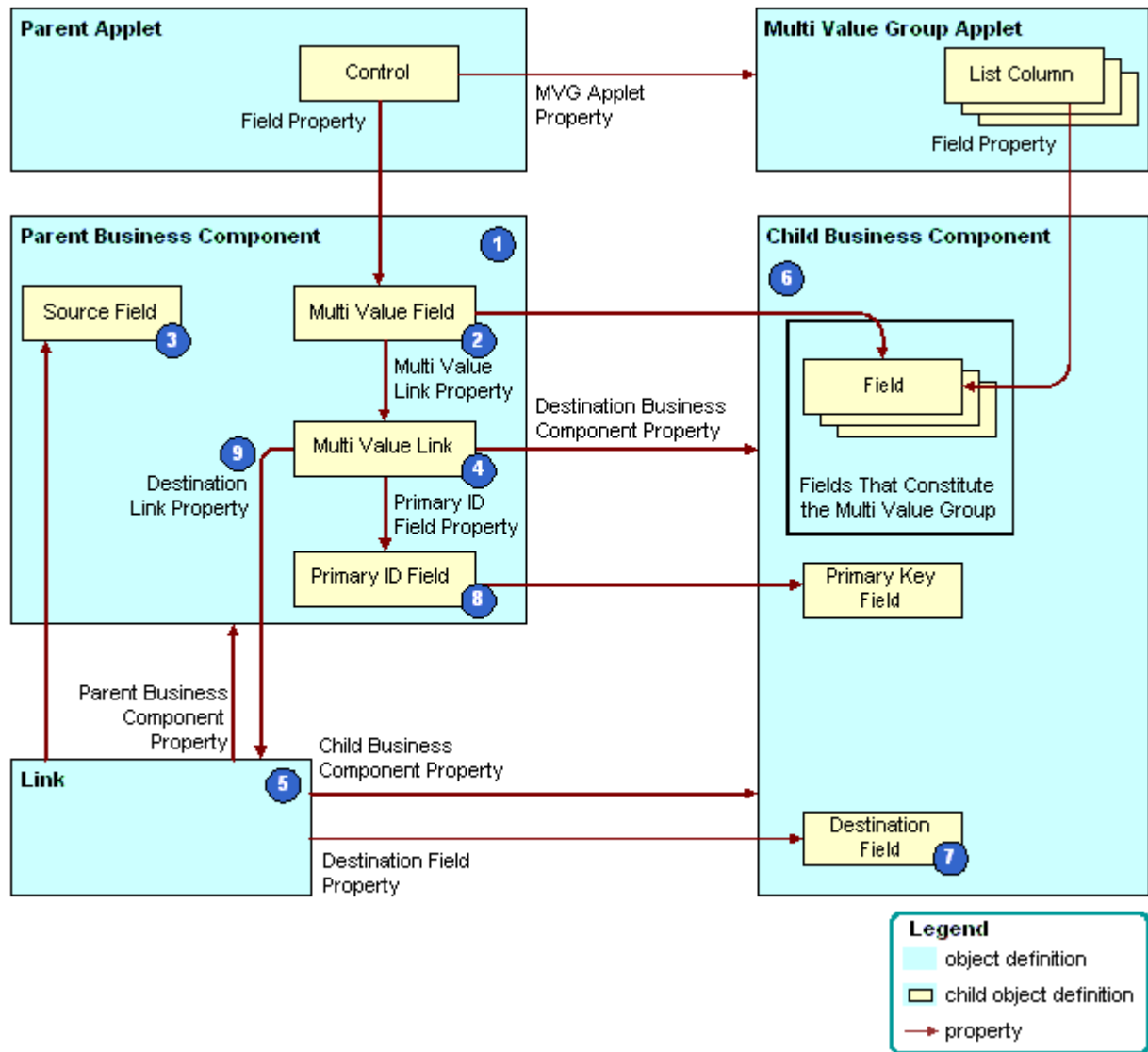
Figure 19. How Siebel CRM Creates a Direct Multi-Value Link
