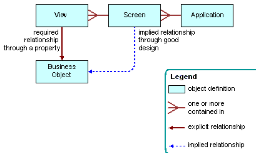
Figure 25. Relationships and Objects That Siebel CRM Uses with a Business Object, Screen, and View
