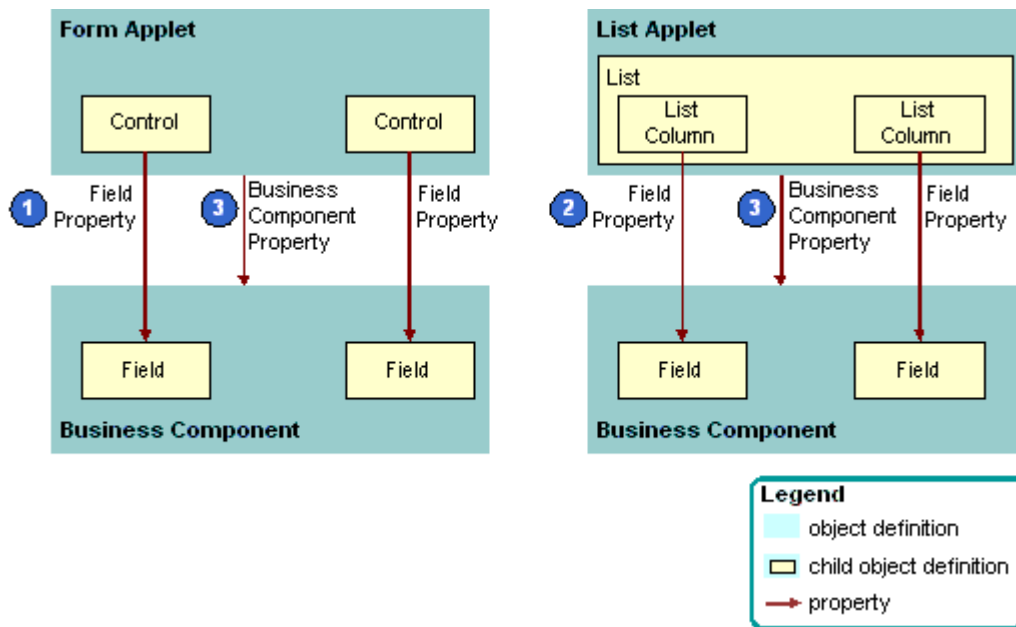
Figure 15. Comparison Between How a Form Applet and a List Applet Reference a Business Component
