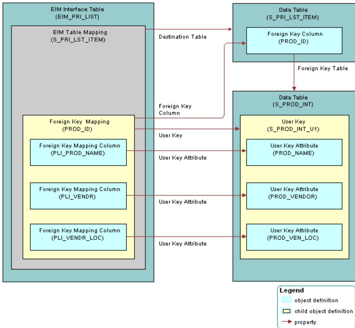
Figure 91. Example of How a Foreign Key Map References a Data Table
