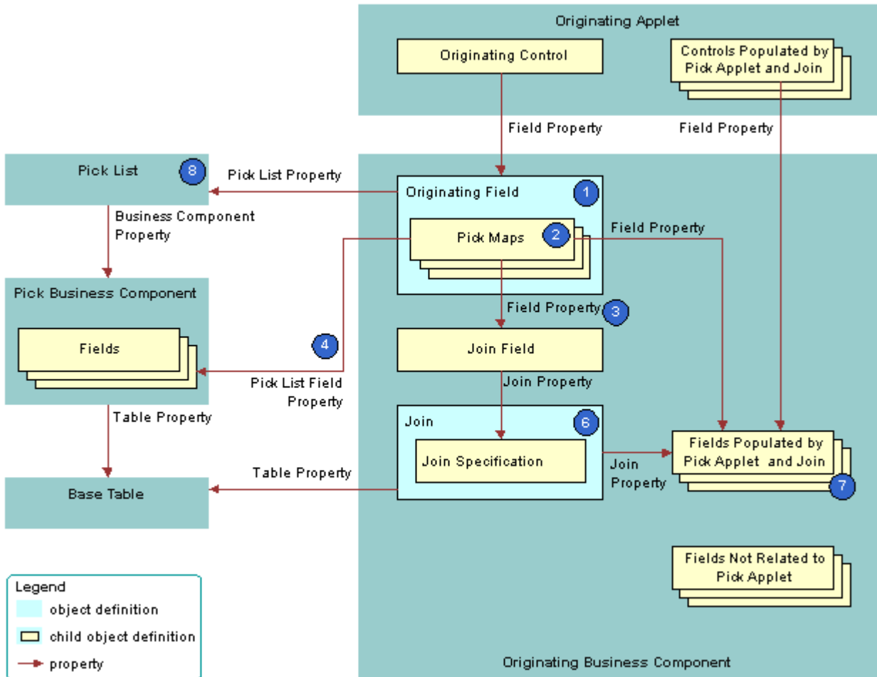
Figure 77. Originating Business Component of a Dynamic List
