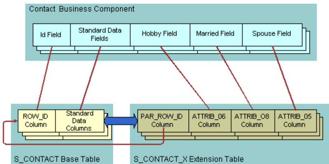
Figure 4. Example of How a One-To-One Extension Table Extends Data Storage for a Single Business Component
