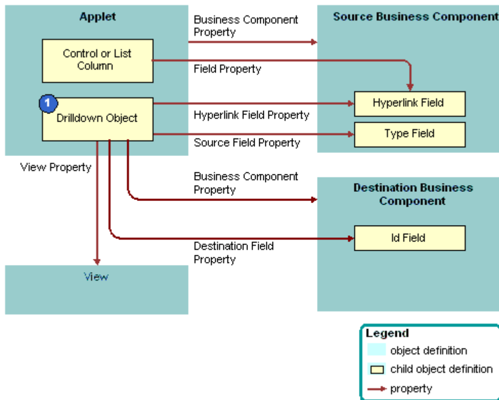
Figure 34. How Siebel CRM Creates a Static Drilldown
