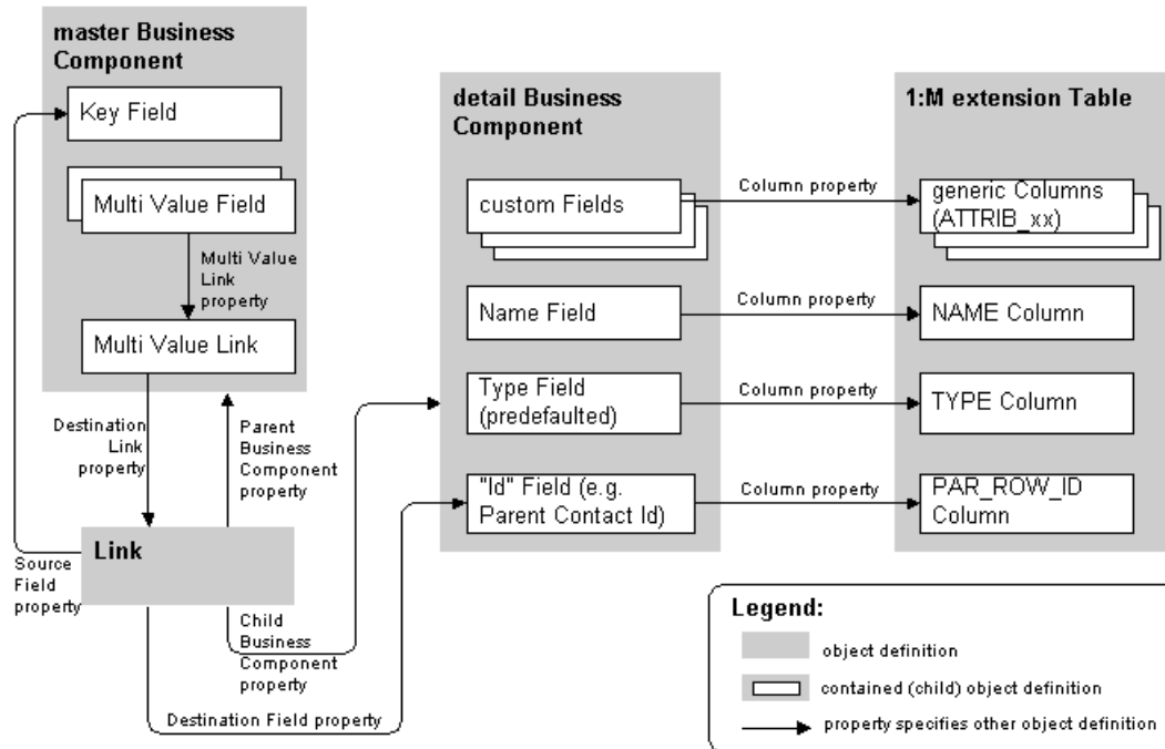
Figure 13. One-to-Many Extension Table Details
