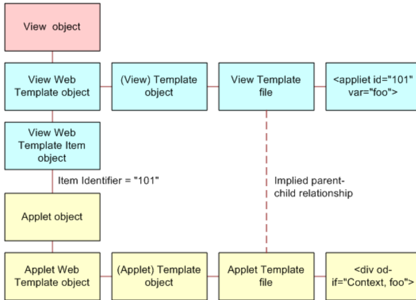
Figure 39. Object Relationships Siebel CRM Uses with the Variable Conditional Tag
