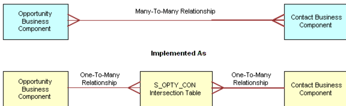
Figure 7. Example of How an Intersection Table Defines a Many-to-Many Relationship
