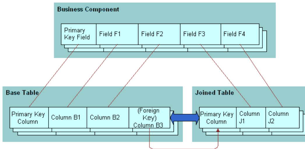
Figure 11. How Fields in a Business Component Reference Columns in a Base Table and a Joined Table
