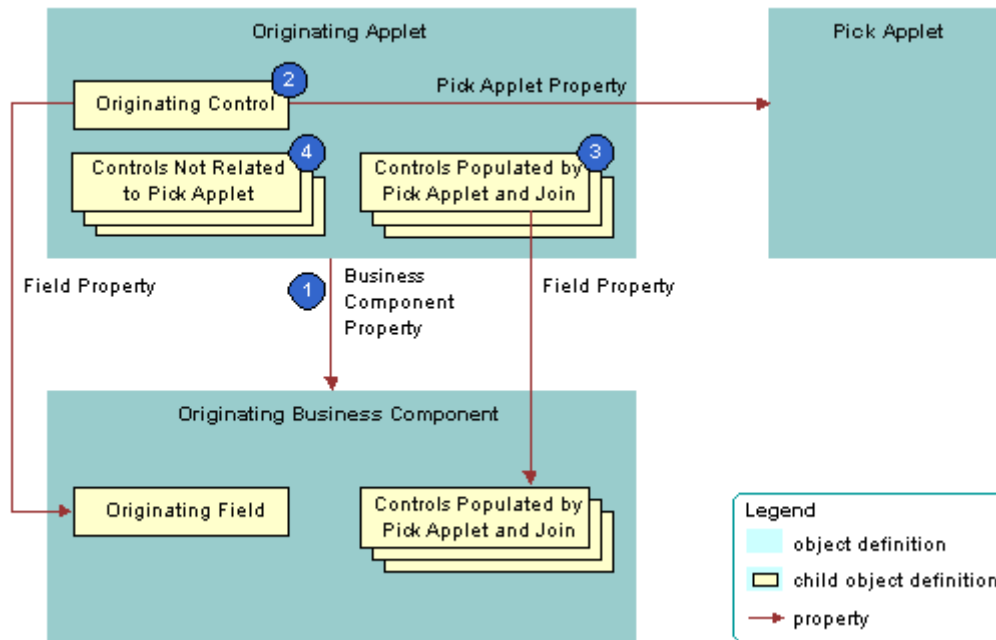
Figure 76. Originating Applet of a Dynamic List
