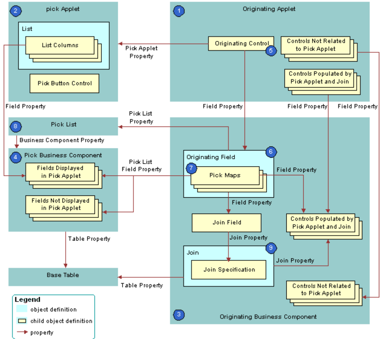
Figure 75. Objects That Siebel CRM Uses to Create a Dynamic List
