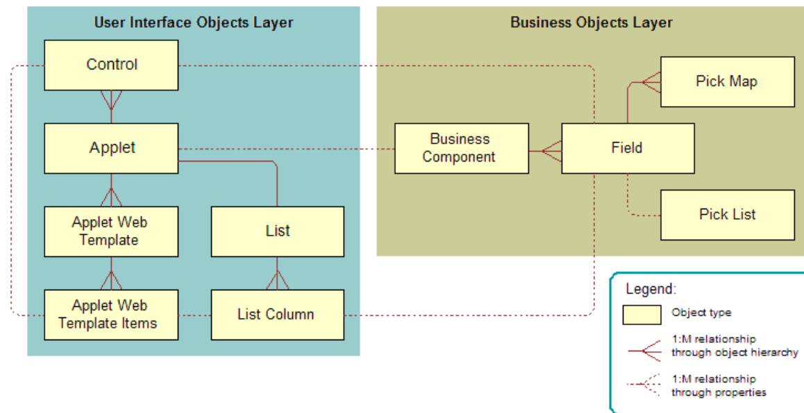
Figure 69. Relationships and Objects That Siebel CRM Uses to Create a Static List
