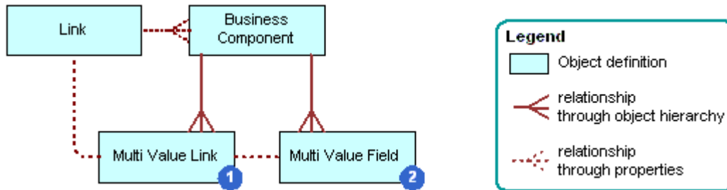
Figure 20. Multi Value Link Architecture
