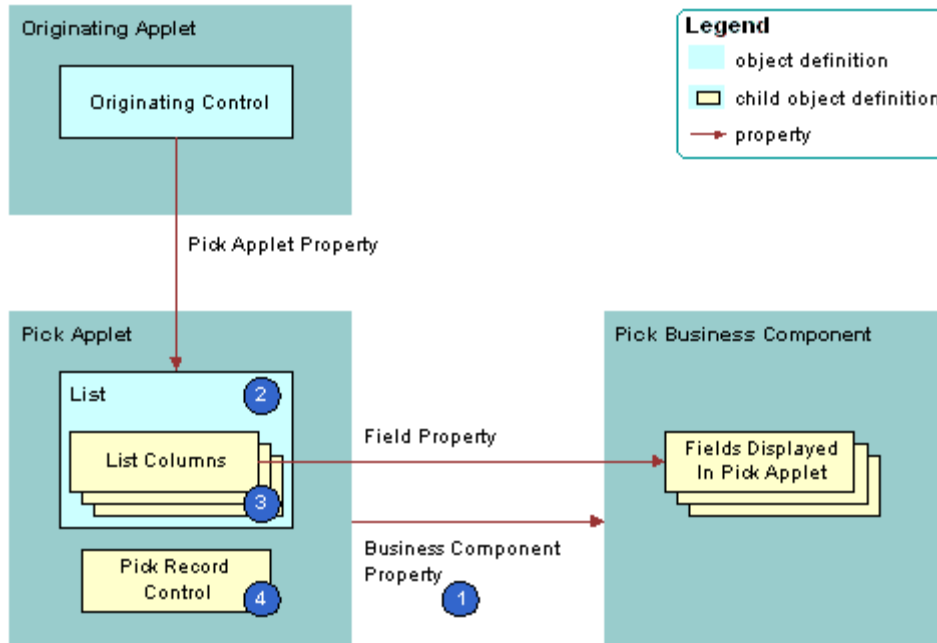
Figure 72. How Siebel CRM Creates a Pick Applet
