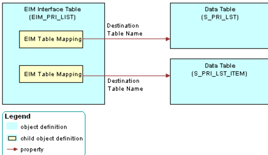
Figure 89. Example of How an EIM Interface Table References a Data Table
