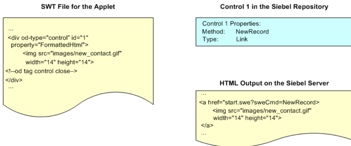
Figure 38. Example of Mappings Between Controls and IDs
