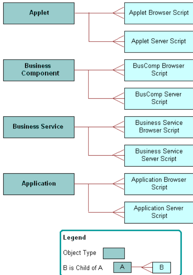
Figure 40. Hierarchy of Relationships Between Object Types That Siebel CRM Uses with a Script
