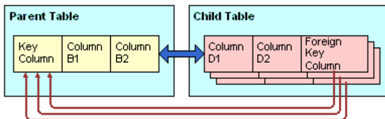
Figure 17. Parent-Child Relationship in a Join
