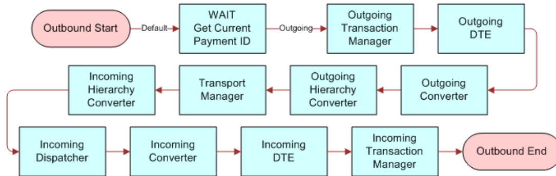
Figure 5. IFX Add Payment Outbound Workflow
