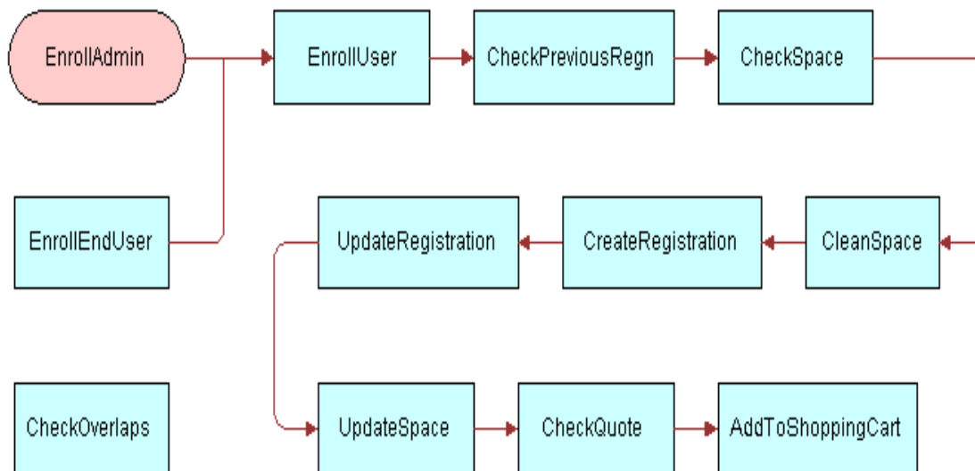
Figure 9. SessionRegistrationService Flow
