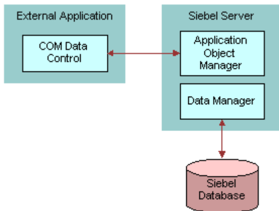
Figure 1. How an External Application Uses COM Data Control
