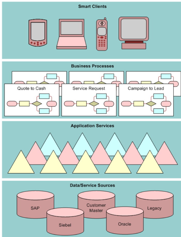
Figure 1. Service-Oriented Architecture
