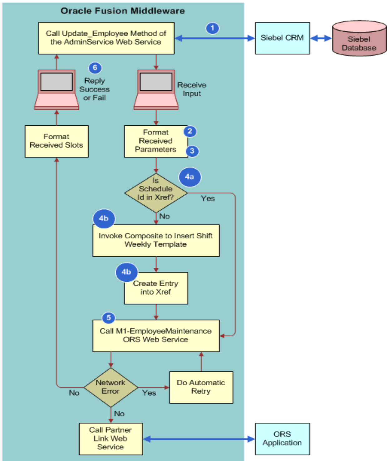
Figure 8. Integration Flow to Update or Insert an Employee Record
