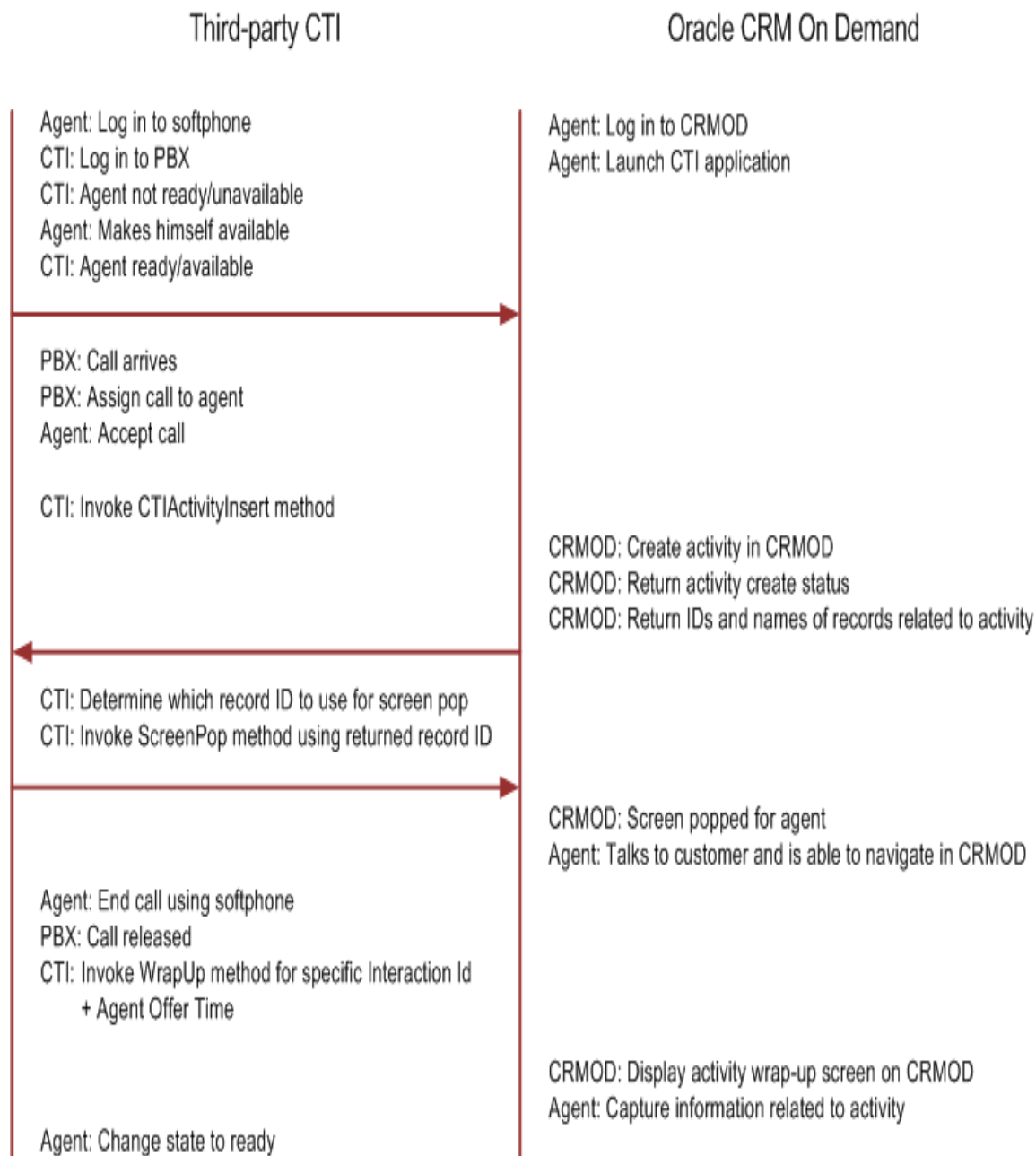
Figure 3. Message Flow
