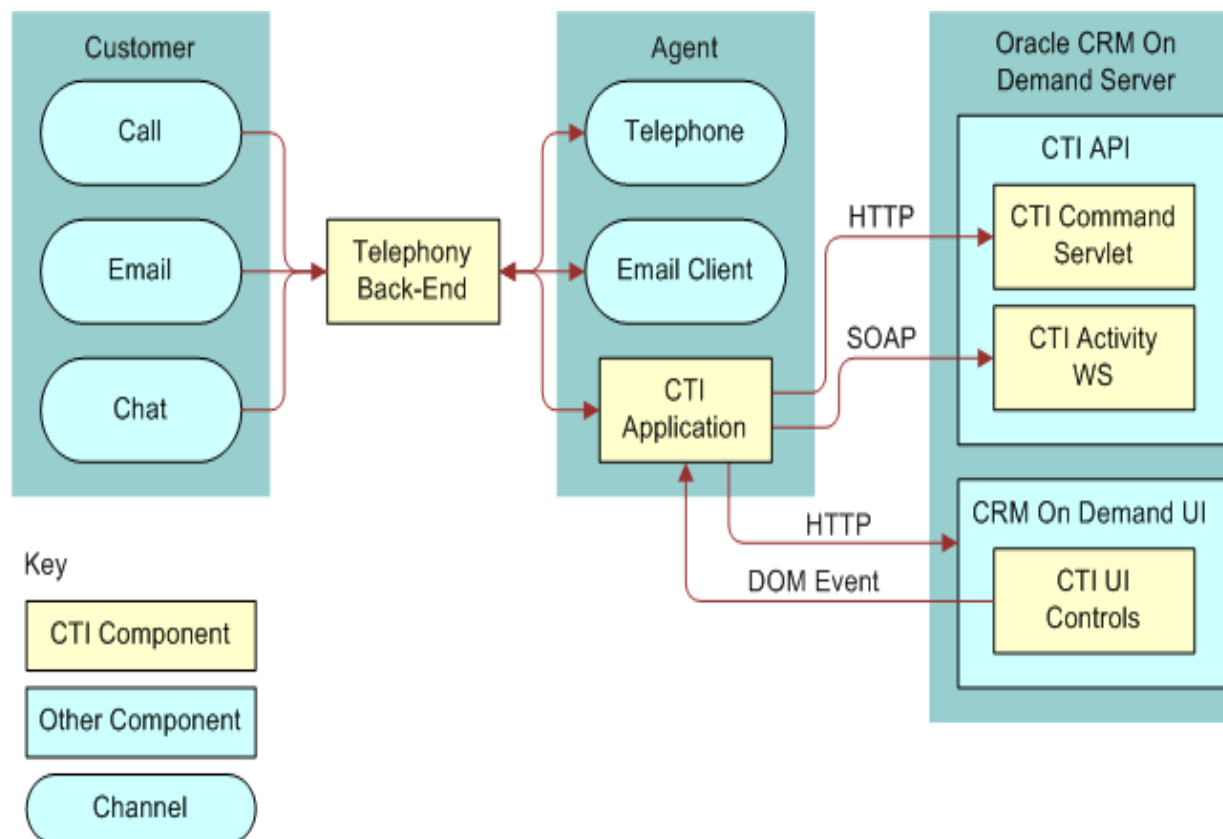
Figure 1. CTI Integration Architecture
